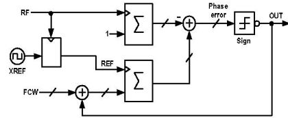
Figure 8. The Divider-less first order \Sigma\Delta Frequency Discriminator
