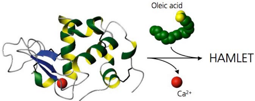
Figure 3. Schematic figure of HAMLET formation. HAMLET consists of \alpha -lactalbumin and oleic acid. The protein is partially unfolded by removal of the calcium ion, which enables oleic acid binding. Structures from pdbID 1HML [54] and 1LFO [86] were modified in MOLMOL [55].
