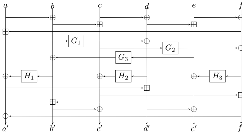
Figure 8.1: F -function.
