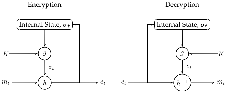
Figure 2.3: General structure of a self-synchronizing stream cipher.
