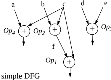
Figure 5. A simple DFG
