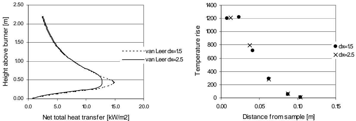
Figure 43. Node dependencies when using the second order accurate TVD numerical scheme based on van Leer and wall-adjacent nodes sizes in the direction normal to the surface of 1.5 cm and 2.5 cm respectively. To the left is the net total heat flux, which is a parameter used directly in flame spread modelling, and to the right the gas temperature in the direction normal to the sample at a location about 0.5 meters above the burner edge.
