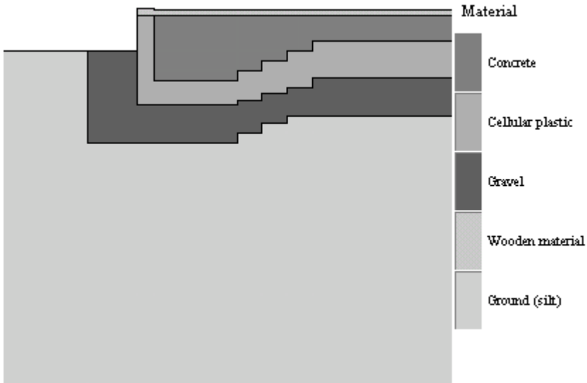
Figure D:2 Drawing/Sketch of the foundation in HEAT2 for the extension of house VI
