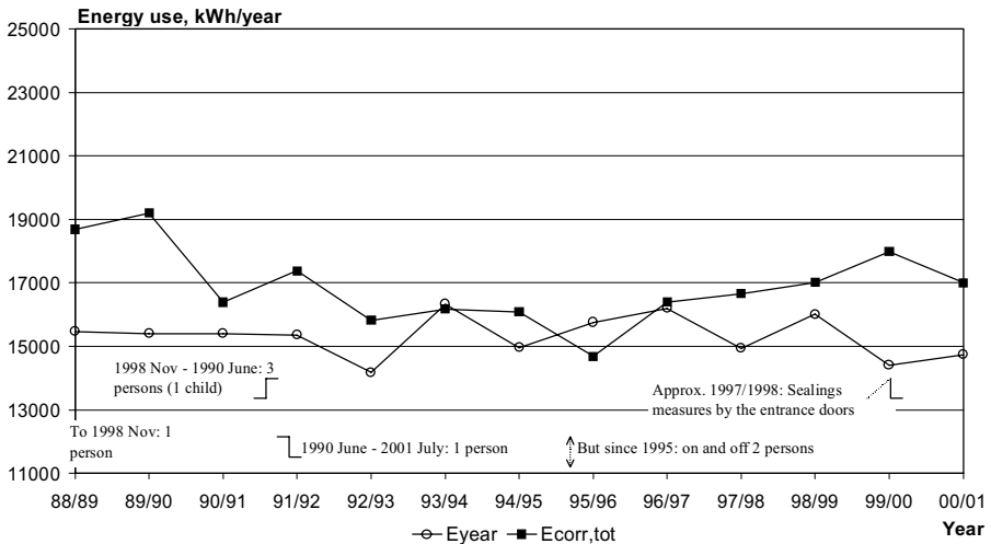
Figure 6:6 Interview answers (including symbols) and yearly energy use from 88/89 to 00/01, House VI
