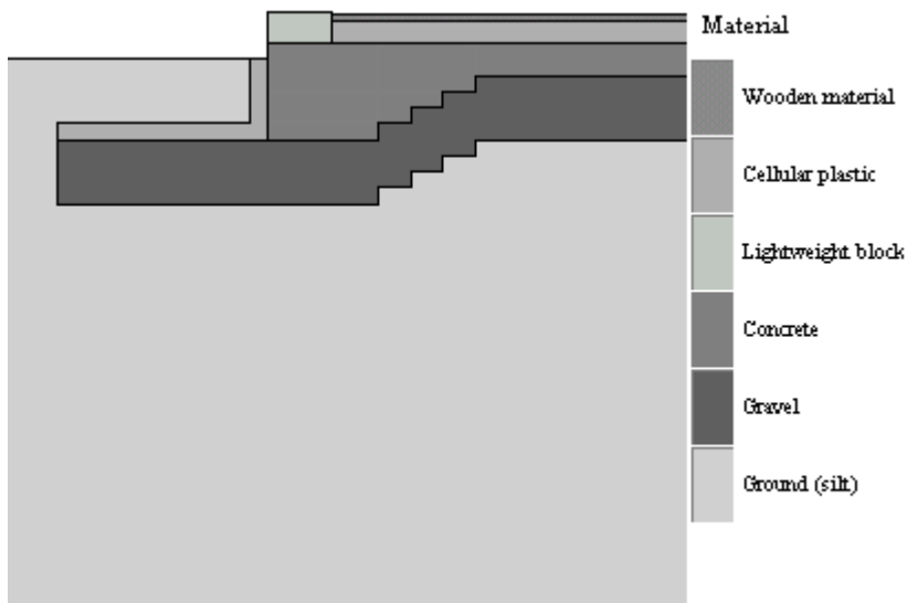
Figure D:1 Drawing/Sketch of the foundation in HEAT2 for the original building
