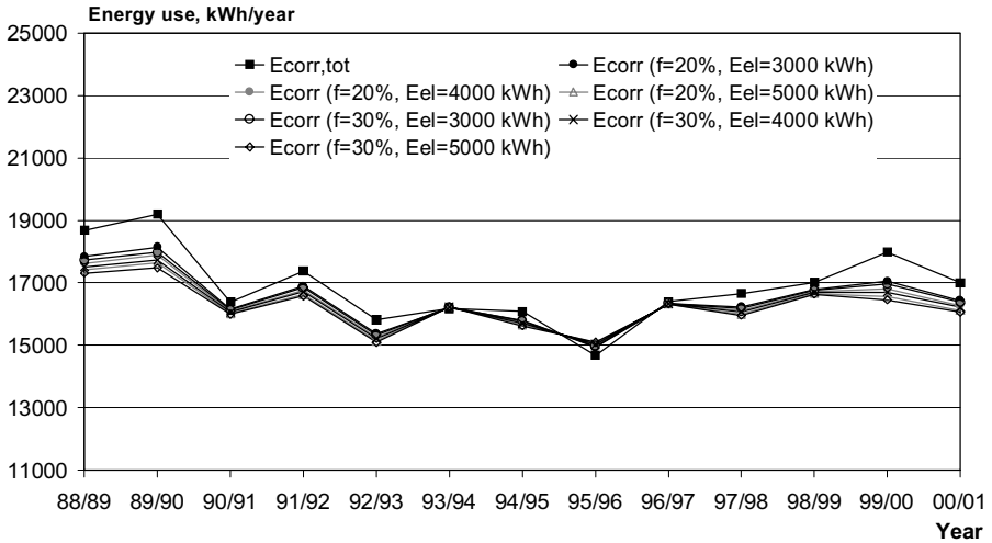
Figure 5:4 Yearly energy use differently corrected ( E_{corr,tot} or f = 20\% , 30\% and E_{el} = 3000, 4000, 5000 kWh) from 88/89 to 00/01, House VI
