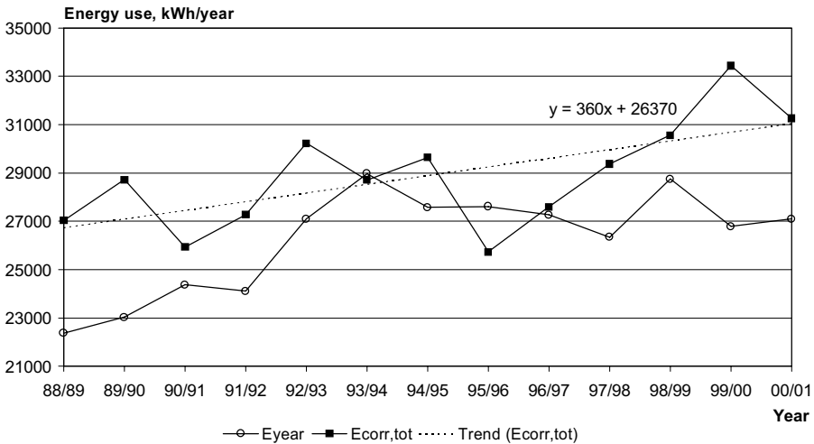
Figure 5:8 Yearly energy use and energy trend from 88/89 to 00/01, House I
