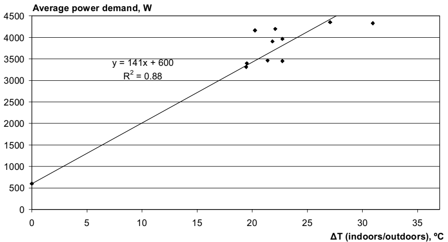
Figure 7:7 Average power demand plotted against temperature difference indoors/outdoors for ten nights including calculated heat loss to the ground, House VI
