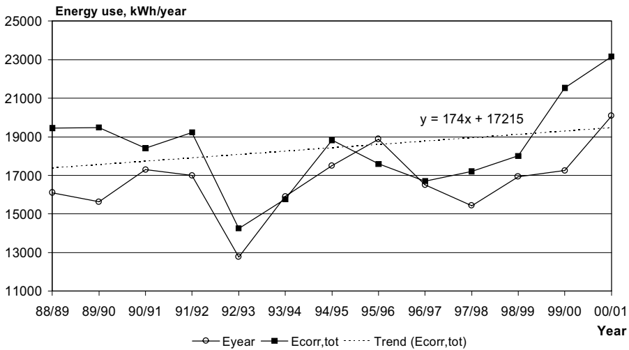
Figure 5:11 Yearly energy use and energy trend from 88/89 to 00/01, House IV
