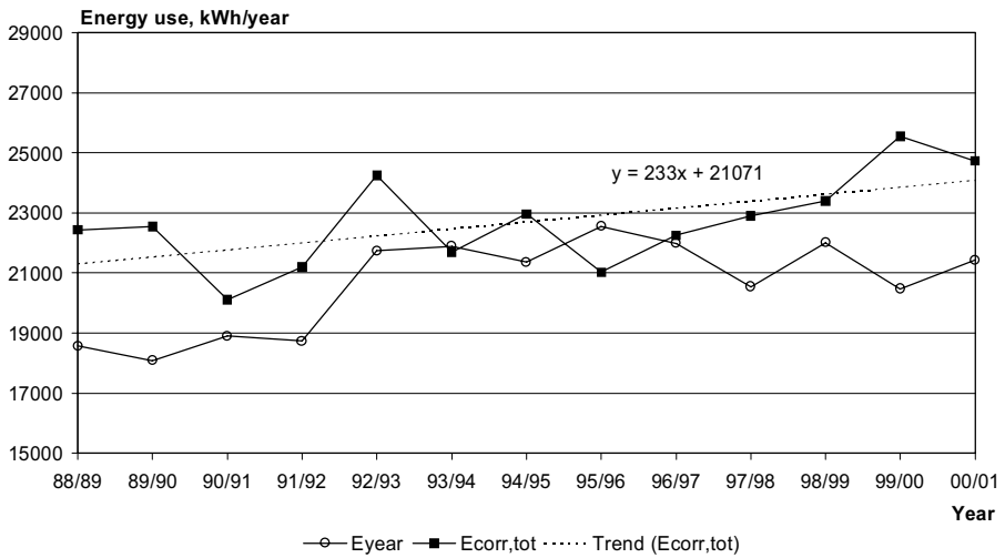
Figure 5:9 Yearly energy use and energy trend from 88/89 to 00/01, House II
