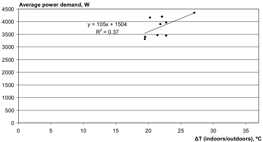
Figure 7:5 Average power demand plotted against temperature difference indoors/outdoors for nine nights, House VI
