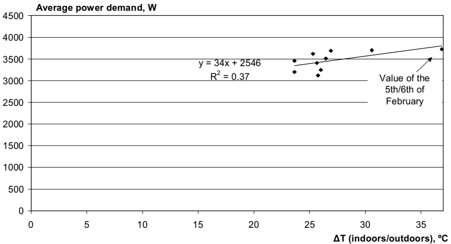
Figure 7:2 Average power demand plotted against temperature difference indoors/outdoors for ten nights, House II
