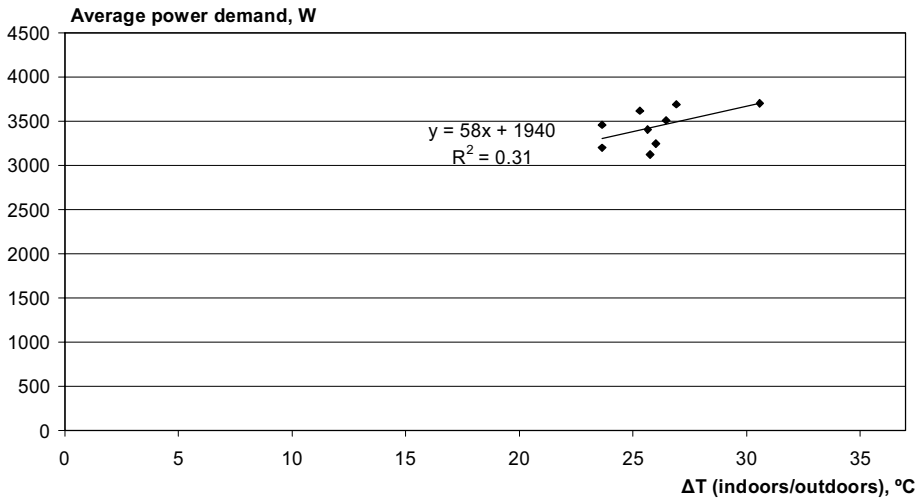
Figure 7:3 Average power demand plotted against temperature difference indoors/outdoors for nine nights, House II
