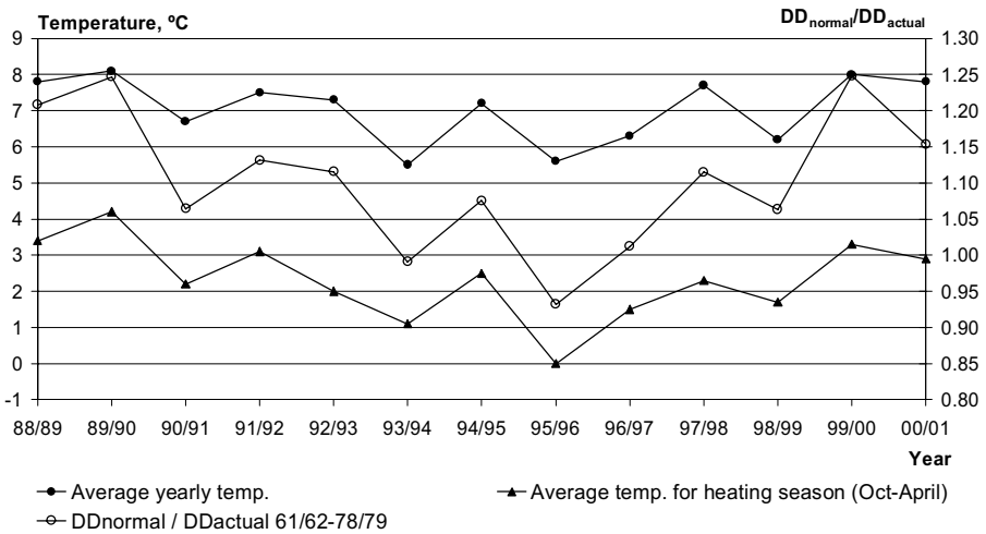
Figure 6:7 The average temperature (yearly and heating season) and degree day correction factor ( DD_{normal}/DD_{actual} ) for the time period 88/89 to 00/01
