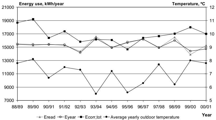
Figure 5:2 Yearly energy use (read of the meter and corrected) and average yearly temperature from 88/89 to 00/01, House VI
