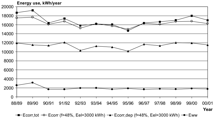
Figure 5:5 Yearly energy use, total or fractions, from 88/89 to 00/01, House VI
