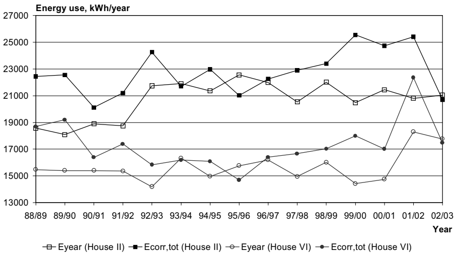
Figure 7:1 Yearly energy use, E_{year} and E_{corr,tot} , from 88/89 to 02/03 for Houses II and VI
