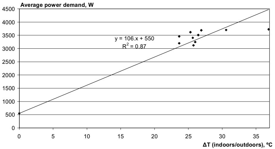
Figure 7:6 Average power demand plotted against temperature difference indoors/outdoors for ten nights including calculated heat loss to the ground, House II
