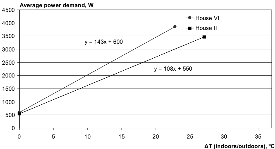
Figure 7:8 An average value of measured power demands plotted against an average temperature difference (indoors/outdoors) including calculated heat loss to the ground, House II and VI
