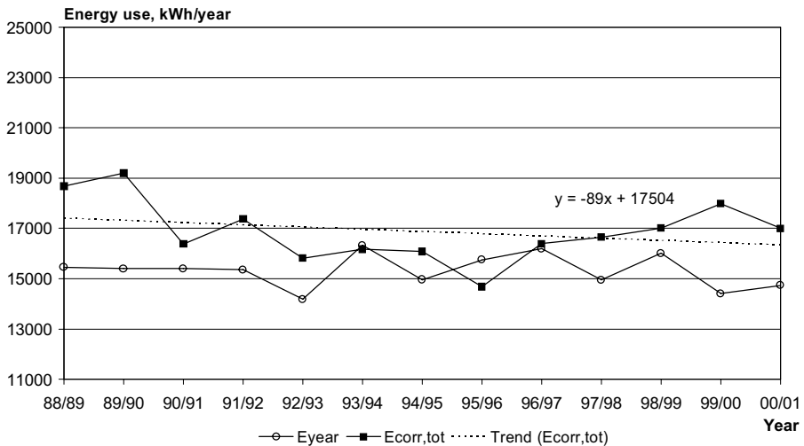
Figure 5:13 Yearly energy use and energy trend from 88/89 to 00/01, House VI
