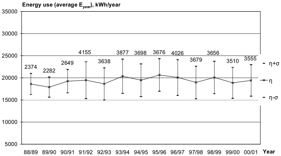
Figure 5:16 Mean ( \eta ) energy use of E_{year} and standard deviation ( \sigma ) for 38 houses from 88/89 to 00/01
