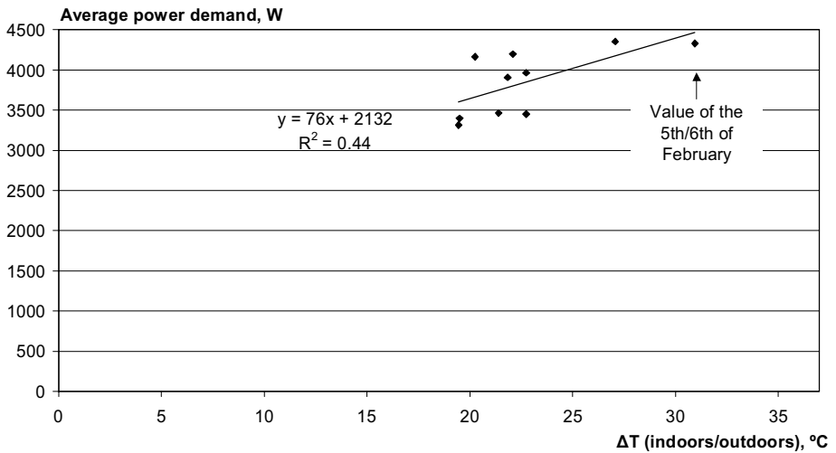
Figure 7:4 Average power demand plotted against temperature difference indoors/outdoors for ten nights, House VI
