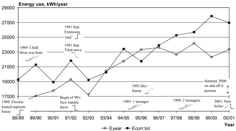
Figure 6:5 Interview answers (including symbols) and yearly energy use from 88/89 to 00/01, House V
