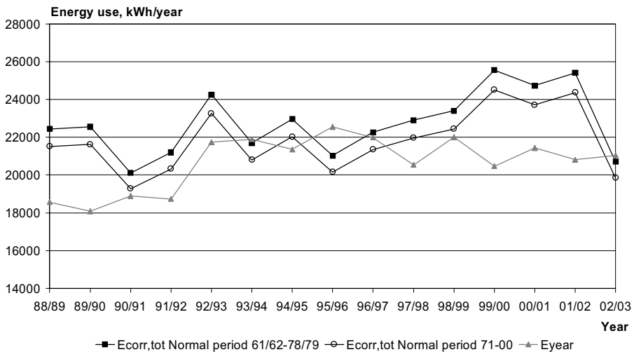
Figure 5:7 Yearly energy use corrected with different normal periods from 88/89 to 02/03, House II
