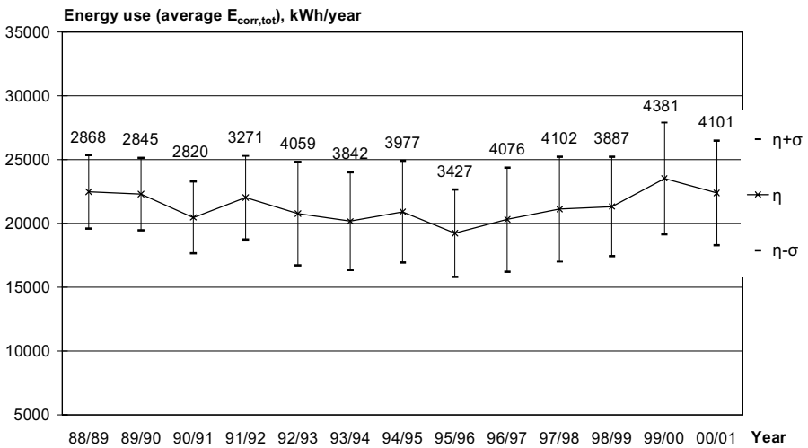
Figure 5:17 Mean ( \eta ) energy use of E_{corr,tot} and standard deviation ( \sigma ) for 38 houses from 88/89 to 00/01
