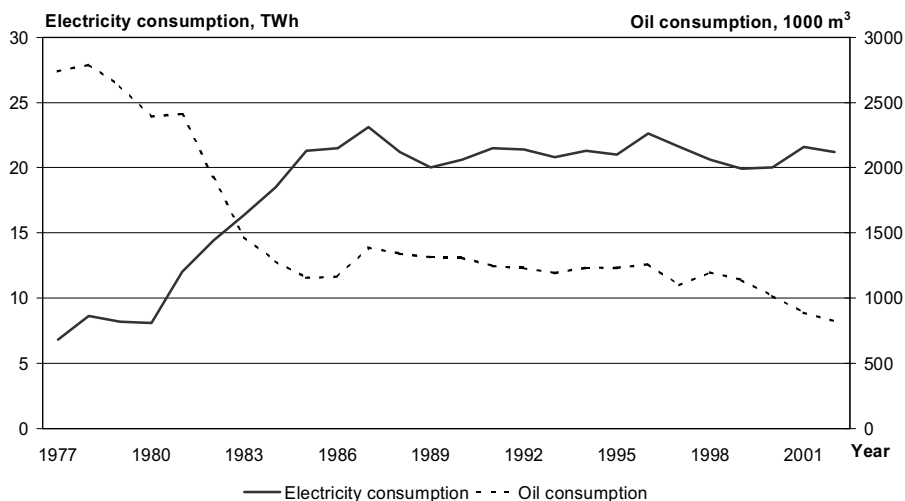
Figure 1:1 Electricity and oil consumption from 1977 to 2002 in single-family houses in Sweden 2,3
