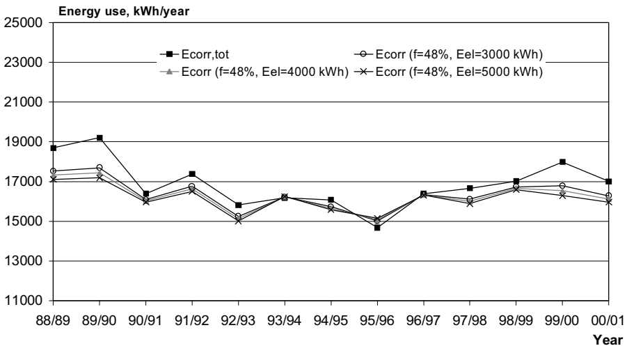
Figure 5:3 Yearly energy use differently corrected ( E_{corr,tot} or f = 48\% and E_{el} = 3000, 4000, 5000 kWh) from 88/89 to 00/01, House VI
