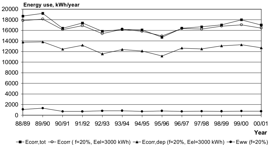
Figure 5:6 Yearly energy use, total or fractions, from 88/89 to 00/01, House VI
