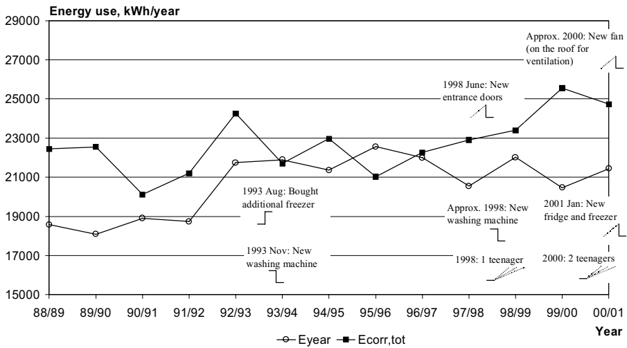
Figure 6:2 Interview answers (including symbols) and yearly energy use from 88/89 to 00/01, House II
