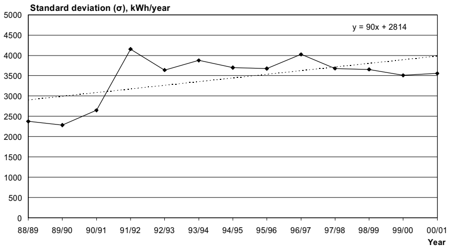
Figure 5:18 Trend of standard deviation ( \sigma ) calculated from E_{year} for 38 houses from 88/89 to 00/01
