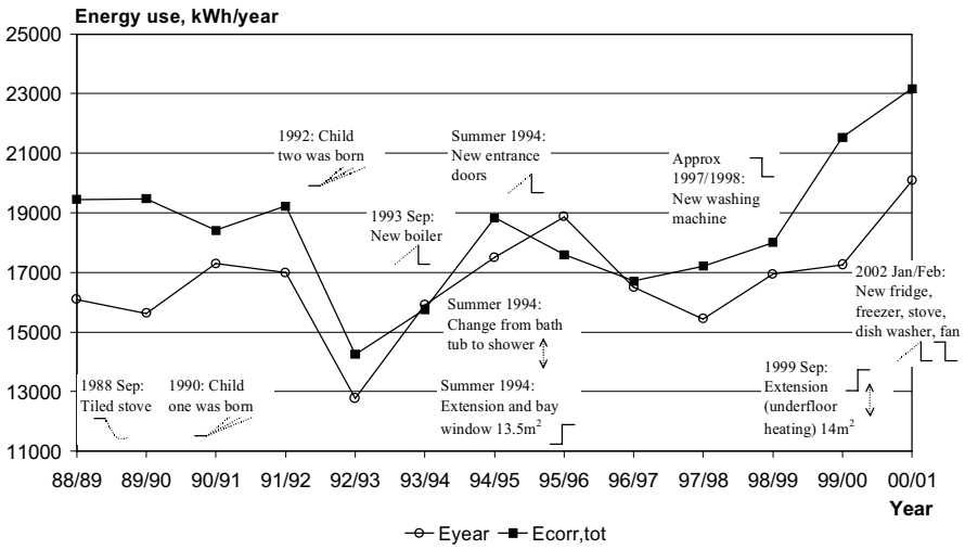
Figure 6:4 Interview answers (including symbols) and yearly energy use from 88/89 to 00/01, House IV
