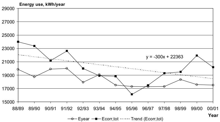
Figure 5:10 Yearly energy use and energy trend from 88/89 to 00/01, House III
