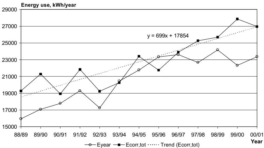
Figure 5:12 Yearly energy use and energy trend from 88/89 to 00/01, House V
