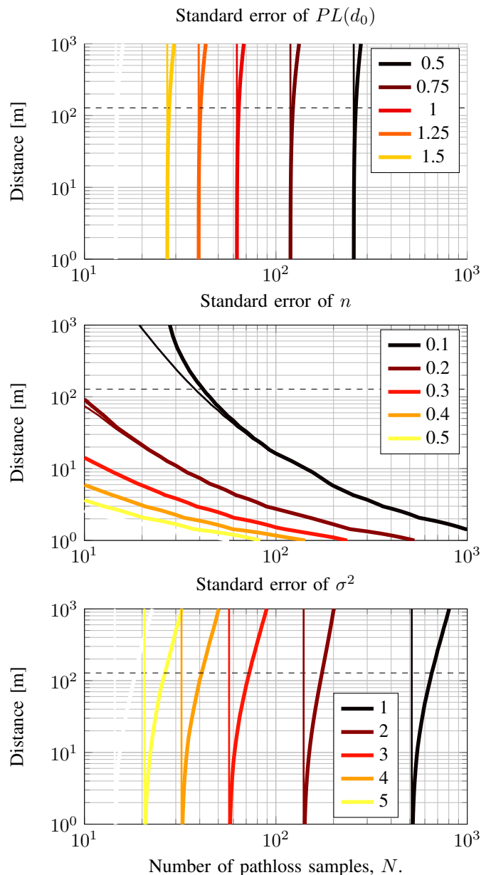
Fig. 2. Standard errors for pathloss parameters estimated with the ML estimator, with the same conditions as in Fig. 2, except that the data is sampled at equally spaced distances on a logarithmic scale, starting from 1 m.
