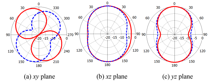
Fig. 6. Radiation patterns of the reconfigurable antennas at 0.87 GHz: (—) bezel mode, (---) fundamental chassis mode.
