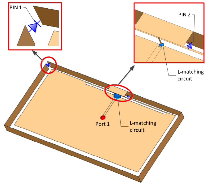
Fig. 3. Geometries of the pattern reconfigurable handset antenna.
