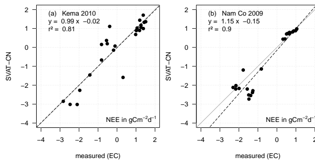
Figure B4. Comparison of hourly medians (see Fig. D3) of measured and modelled net ecosystem exchange for the 2010 campaign at Kema (left panel) and 2009 campaign at Nam Co (right panel). The regression line (dashed, black) is shown as well as the 1 : 1 line (solid, grey).
