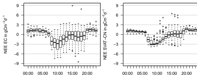
Figure B3. Mean diel course of measured (left panel) and modelled (tile approach according to the EC footprint: S_{\text{RefEC}} , right panel) net ecosystem exchange (NEE) over 61 days of 2010 (3 June to 2 August) at Kema: box plot with median, 25 % and 75 % quartiles; bars represent quartiles \pm 1.5 times interquartile range, dots are outliers. Measured and modelled values are restricted to high data quality (flag 1–3 out of a scheme ranging from 1 to 9, Foken et al., 2004).
