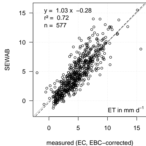
Figure B1. Scatter plot of measured vs. SEWAB modelled S_{\text{RefEC}} evapotranspiration (ET) over 61 days of 2010 (3 June to 2 August) at Kema. Measured and modelled values are restricted to high data quality (flag 1–3 out of a scheme ranging from 1 to 9, Foken et al., 2004). Measured EC data is corrected according to the surface energy imbalance with the buoyancy flux correction.
