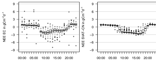
Figure B5. Mean diel course of measured (left panel) and modelled (right panel) net ecosystem exchange (NEE) over 44 days during 2009 (26 June to 8 August) at Nam Co: box plot with median, 25 and 75 % quartiles; bars represent quartiles \pm 1.5 times interquartile range, dots are outliers. Measured and modelled values are restricted to high data quality (flag 1–3 out of a scheme ranging from 1 to 9, Foken et al., 2004). Model parameters for leaf physiology and soil respiration were adapted for best representation of eddy-covariance data (see Sect. 3.2.1).
