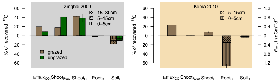
Figure 7. 13 C partitioning and distribution of recently allocated C within the various pools, namely CO 2 efflux, shoot respiration, shoots, roots and soil for Xinghai site (grazed and ungrazed) in 2009 and Kema site (IM) in 2010, determined at the end of a 29 day and 15 day allocation period, respectively. Vertical lines in the bars denote standard errors ( n = 3 for Xinghai 2009 and n = 8 for Kema 2010). Total fluxes of C in \text{g C m}^{-2} \text{d}^{-1} to the different C pools at Kema site are based on the combination of eddy-covariance measurements and labelling. Shoot respiration is not measured, but determined as difference between the 13 C recovery at the first sampling and the sampling at the end of the allocation period. First sampling in Xinghai was 1 day after the labelling and in Kema at the labelling day. Figure modified after Hafner et al. (2012) and Ingrisch et al. (2014).
