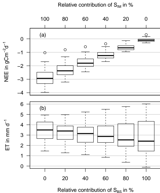
Figure 9. Modelled daily net ecosystem exchange (top, NEE) and modelled daily evapotranspiration (bottom, ET) for 46 days (12 July to 26 August 2012) at Kema (varying combination of S_{IM} and S_{BS} ): box plot with median, 25 % and 75 % quartiles; bars represent quartiles \pm 1.5 times interquartile range.
