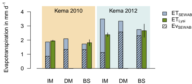
Figure 3. Evapotranspiration (ET) derived with SEWAB and with micro-lysimeter measurements at Kema in 2010 (33 days: 23 June–25 July) and Kema in 2012 (40 days: 16 July–24 August) for intact root mat (IM), degraded root Mat (DM) and bare soil (BS). Hatched bars denote the simulated evaporation (Ev) as part of the total simulated ET, the remainder is transpiration. Black lines on top of the bars for the micro-lysimeter illustrate standard deviations ( n = 4 ).
