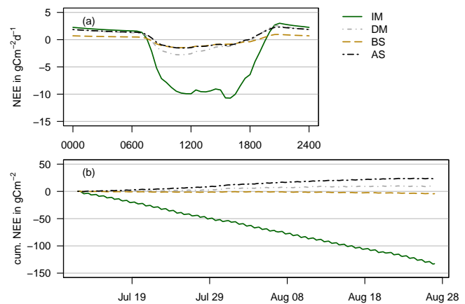
Figure 6. Model results of net ecosystem exchange (NEE) over 46 days of July and August 2012 at Kema. (a): mean diurnal cycle, and (b): cumulative NEE. The four lines represent different stages of vegetation degradation (IM, DM, BS, and AS).
