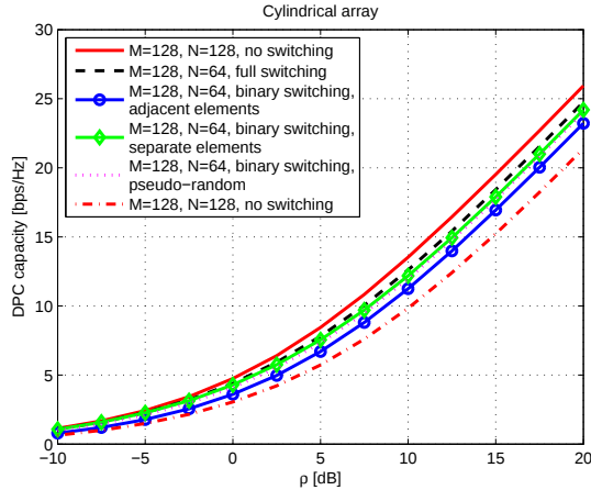
Fig. 8. Performance comparison in the LOS scenario where four users are closely located at MS 2, with the cylindrical array at the base station.
