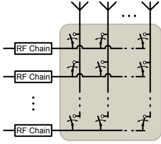
Fig. 1. A symbolic illustration of a full switching network.
