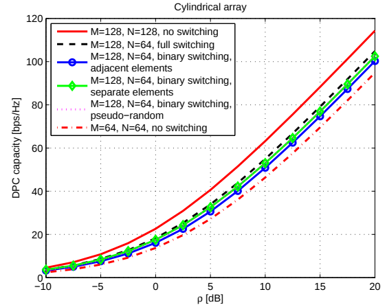
Fig. 10. Performance comparison in the scenario where sixteen users are distributed at MS 1-8, half have LOS conditions and half have NLOS conditions, with the cylindrical array at the base station.
