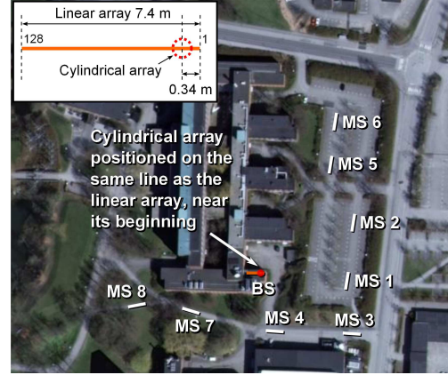
Fig. 4. Overview of the measurement area at the campus of the Faculty of Engineering (LTH), Lund University, Sweden. The two base station antenna arrays were placed on the same roof of the E-building during two measurement campaigns. Eight sites around the E-building were measured.
