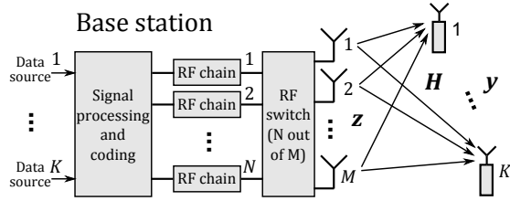
Fig. 5. System model of a multi-user MIMO system with transmit antenna selection.
