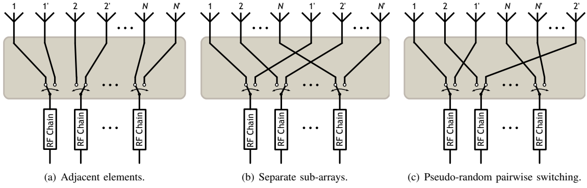
Fig. 6. Three example configurations of the proposed binary switching solution (for M = 2N ).
