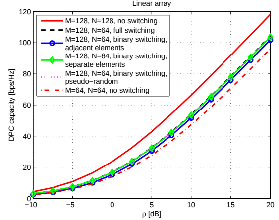
Fig. 9. Performance comparison in the scenario where sixteen users are distributed at MS 1-8, half have LOS conditions and half have NLOS conditions, with the linear array at the base station.
