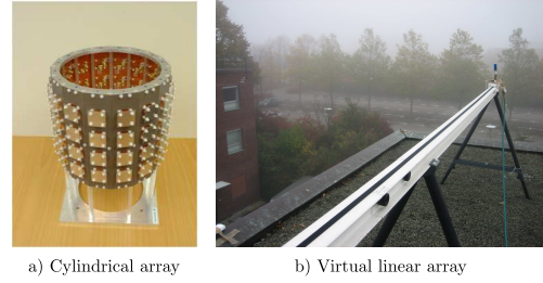
Fig. 3. Two large antenna arrays at the base station side: a) a cylindrical array with 64 dual-polarized patch antennas, giving 128 ports in total, and b) a virtual linear array with 128 vertically-polarized omni-directional antennas.
