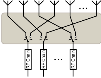
Fig. 2. A binary switching network.
