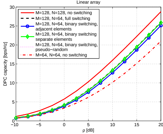
Fig. 7. Performance comparison in the LOS scenario where four users are closely located at MS 2, with the linear array at the base station.
