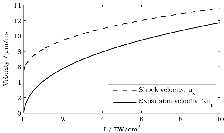
Figure 4.12: Shock and expansion velocity curves for aluminium. For zero laser intensity, the shock velocity equals the sound speed, c_0 , of the material, whereas the expansion velocity goes to zero.
