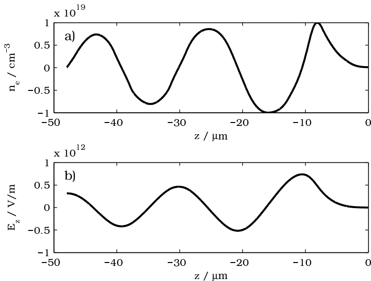
Figure 3.3: The ponderomotive force of the laser pulse (located at around z = -10 \mu\text{m} in the figure, traveling right) pushes electrons out of the focal region. The electrostatic restoring force resulting from the ions sets up an oscillating density variation, as illustrated in a). The longitudinal electric field resulting from this charge density distribution is depicted in b). The peak field strength is approaching 1 TV/m.
