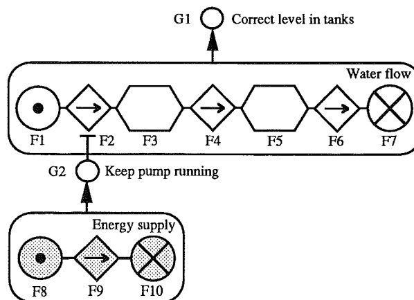
Figure 4.5 An MFM model of the tanks process. The main goal is to keep the level of the upper tank correct, and it is achieved by a water flow. In order for the transport function F2 to be available, i.e., to keep the pump running, energy must be supplied.
