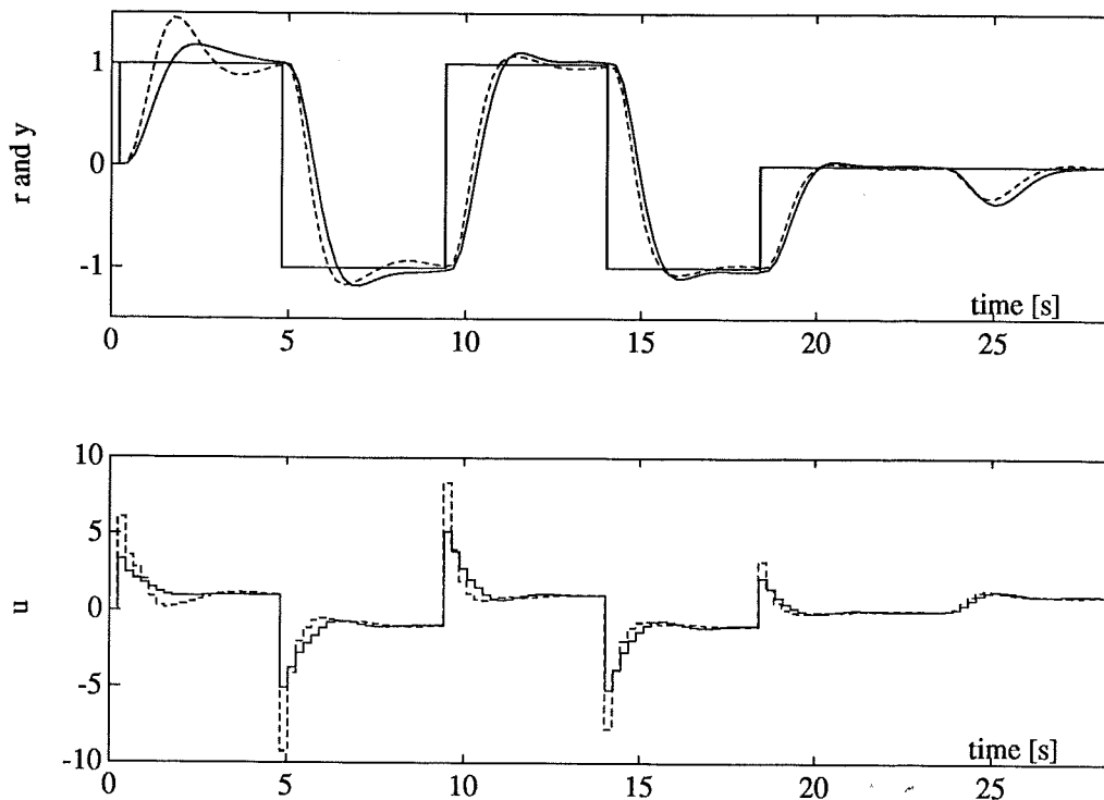
Figure 7.7 Adaptive control of process G_C(s) . The solid curves represent the system based on the second order model. The dashed curves represent the system for the third order model.
