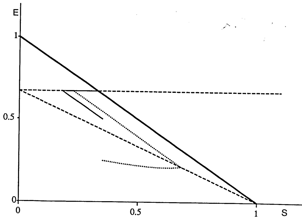
Figure 8.6 Simulation of the time optimal strategy to compensate one small and one large disturbance to the reactor. Below, the trajectory in the state space is shown.
