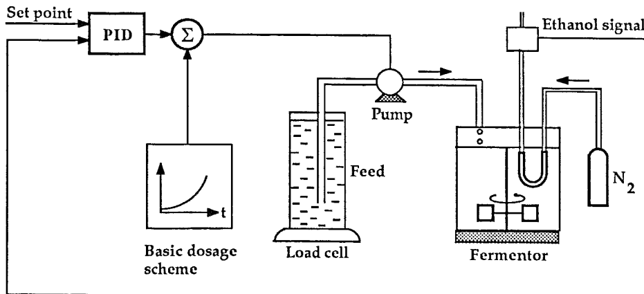
Figure 4.1 Experimental set-up for substrate dosage control.
