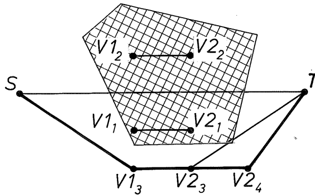
Figure B.7 An example of the search for an obstacle free way in the path finding algorithm. The denotations are: S: starting point of the path, T: terminal point of the path, V1_i, V2_i : vertices of the polygon path. The index i denotes the search order. The obstacle map contains one obstacle, which is situated between S and T. The search has gone as: Path (S,T) not free \rightarrow Path ( V1_1, V2_1 ) not free \rightarrow Path ( V1_2, V2_2 ) not free \rightarrow Path ( V1_3, V2_3 ) free Path (S, V1_3 ) free Path ( V2_3, T ) not free \rightarrow Path ( V2_4, T ) free which results in a free way from S to T.
