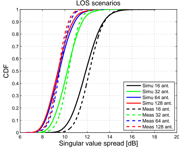
Figure 2: Singular value spreads of the simulated channels and measured channels.
