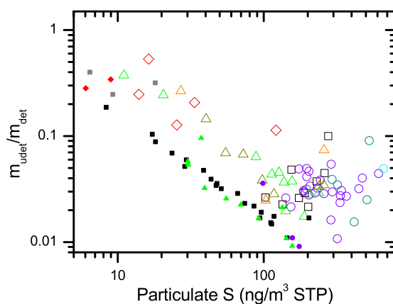
Figure 3.2. Scatter plot of the ratio of the estimated particulate mass of S outside the analytical beam area ( m_{undet} ) to the detected mass ( m_{det} ) as a function of the atmospheric particulate S concentration. Particulate S was detected in the analytical area of all samples. Open symbols indicate cases where S was also detected outside the analytical area, whereas the small, closed symbols denote samples where S was undetected outside the analytical area.
