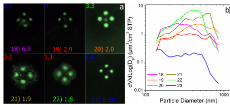
Figure 7. Samples outside the C_V / C_M range of 0.55\text{--}1.55\text{ cm}^3\text{ g}^{-1} marked in Fig. 2 that cannot be connected with cloud, crust or large carbonaceous fraction. (a) Particle deposition patterns on the aerosol samples with measurement No. and C_V / C_M ( \text{cm}^3\text{ g}^{-1} ) at bottom of the images. Numbers in top left corners show deposition pattern and the colour indicates air mass type according to the legend of Fig. 3. (b) Volume size distributions from the OPC.
