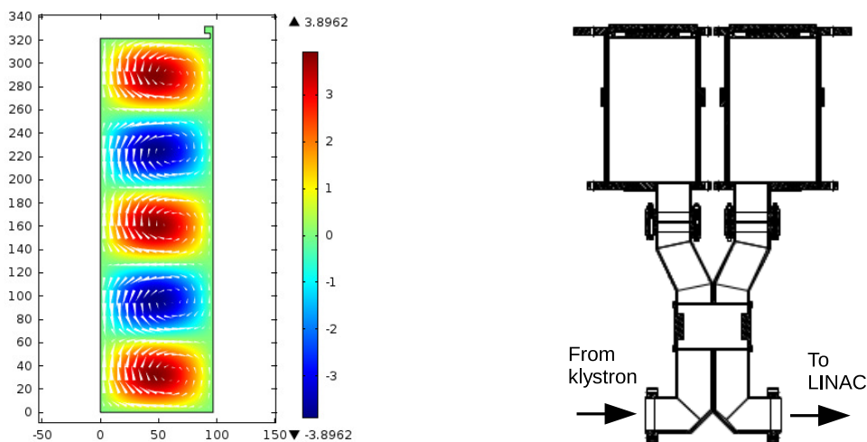
Figure 3: E_\phi(r, \phi, z) (color scale) and Figure 4: The SLED cavities with the \mathbf{H}(r, \phi, z) (white cones) of the \text{TE}_{015} 3dB \pi/2 hybrid coupler mode.
