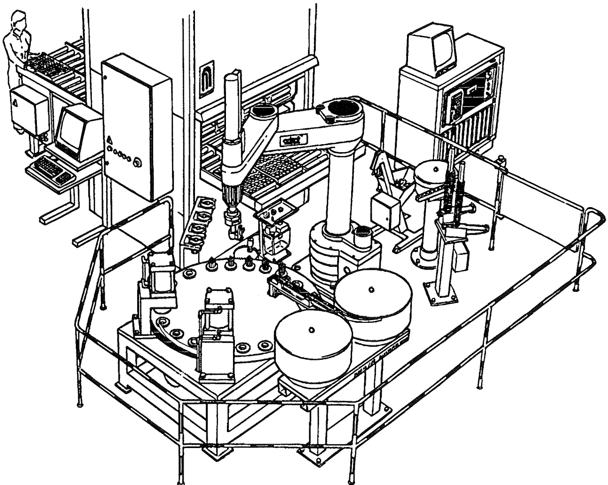
Figure 2.6 An assembly work cell, from [22] with permission from IVF.
