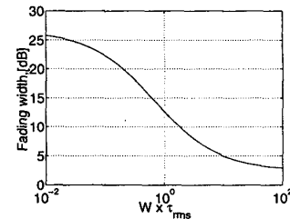
Figure 3. Fading width as a function of the system bandwidth times delay spread (Equation (4.1)) and references [2&3]
