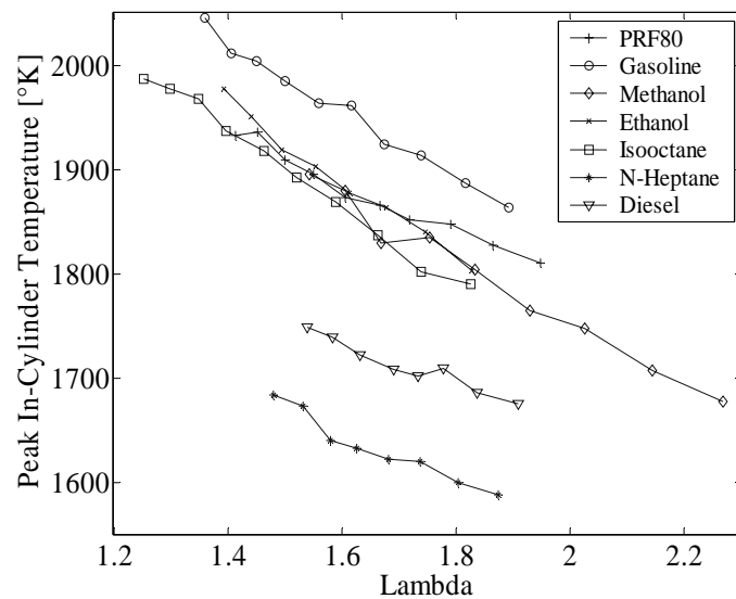
Figure 32. Peak in-cylinder temperature as function of lambda.
