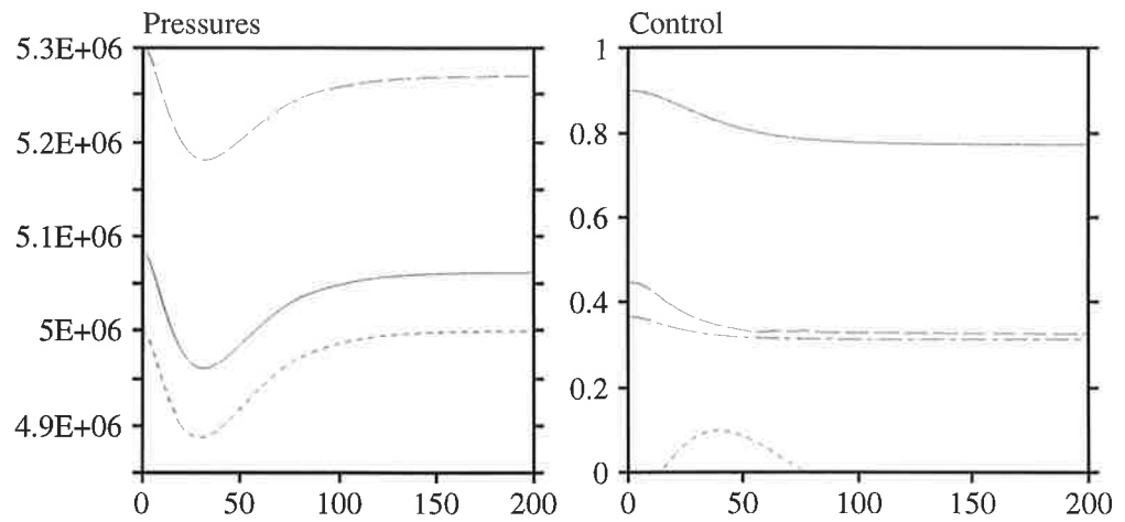
Figure 20. Pressures in the pan and the main control variables with decreasing flue-gas flow. (Solid line - throttle valve, dashed - deaer. valve, dash-dotted - boiler valve, dotted - steam injection valve.)
