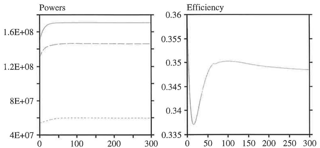
Figure 18. Power and efficiency ( P_{out}/P_{tot} ) with increasing flue-gas flow. From the top: total heat, transferred heat and electrical output.
