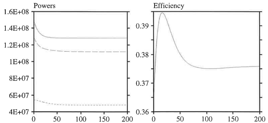
Figure 21. Power and efficiency ( P_{out}/P_{tot} ) with decreasing flue-gas flow. From the top: total heat, transferred heat and electrical output.
