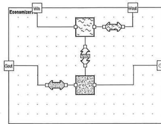
Figure 7. The configuration of a heat exchanger.
