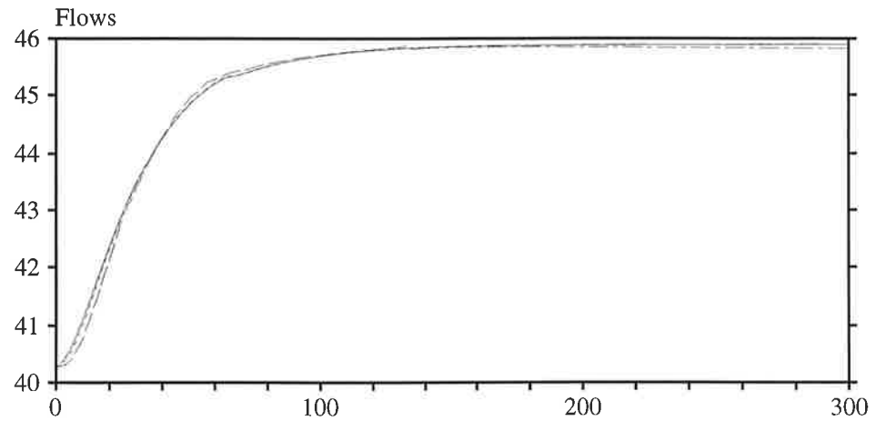
Figure 16. Flow changes when the flue-gas flow increases. (Solid line - steam, dashed - condensate, dotted - feedwater, dash-dotted - turbine flow.)
