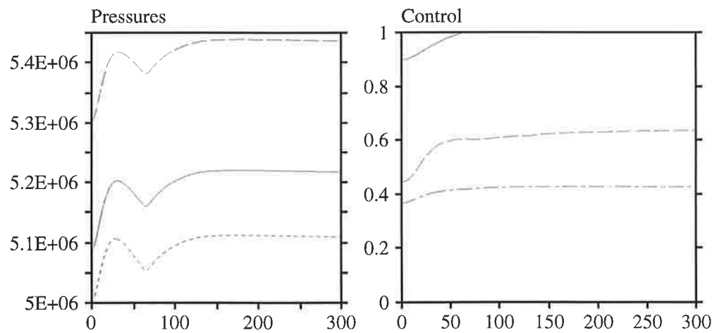
Figure 17. Pressures in the pan and the main control variables with increasing flue-gas flow. (Solid lines - throttle and bypass valves, dashed - deaer.valve, dash-dotted - boiler valve.)
