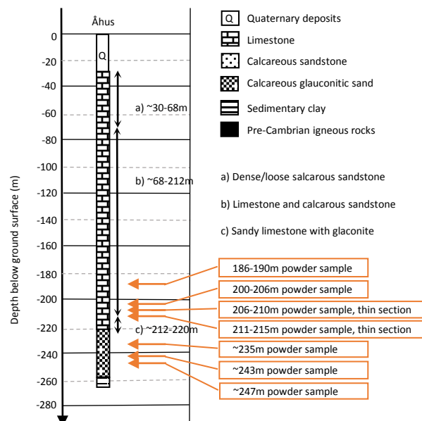
Figure 9. The main geological units in the Åhus core (personal communication, Martin Ekvý, Malmberg Borning, June 2015). The levels where samples were collected and analyzed with SEM and EDS are shown.
