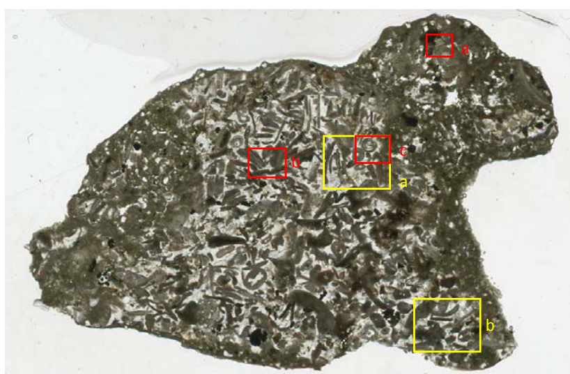
Figure 14. Photograph of the thin section from core level 211-216m. Microscopic photographs of the yellow framed subareas are shown in Fig. 15, and chemical mappings of the red subareas are shown in Figs 16-18.
