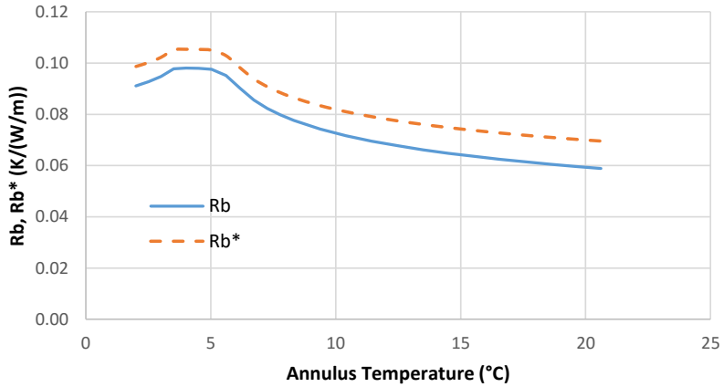
Fig. 5 Borehole thermal resistance and effective borehole thermal resistance for ground-water filled borehole with fixed heat rejection rate, but changing mean fluid temperature
