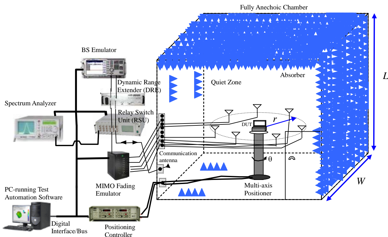
Figure 1.1: Tentative MIMO OTA test system configuration [2].
