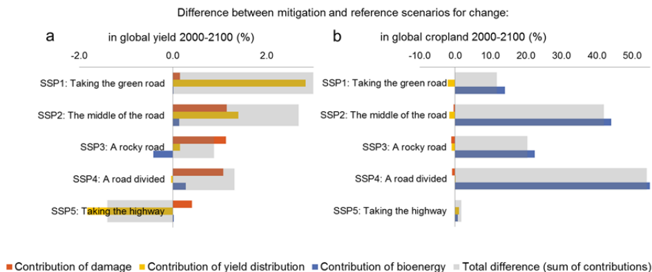
Figure 7: Differences between reference and mitigation scenarios for changes in global yield (2000-2100, %, panel a) and changes in global cropland (2000-2100, %, panel b). The grey bar indicates the total differences (sum of differences due to impacts of changes in damage, yield distribution and bioenergy), while the coloured bars show the contribution of different impacts to the total difference.
