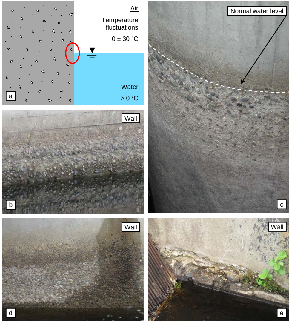
Figure 2-6. Temperature conditions at the waterline are shown in (a). Photos (b–d) show three examples of surface deterioration of concrete at the waterline of hydro power structures. Photos (b–c) are taken on the upstream side whereas photo (d) is taken on the downstream side. Photo (e) shows an example of internal damage above the waterline.
