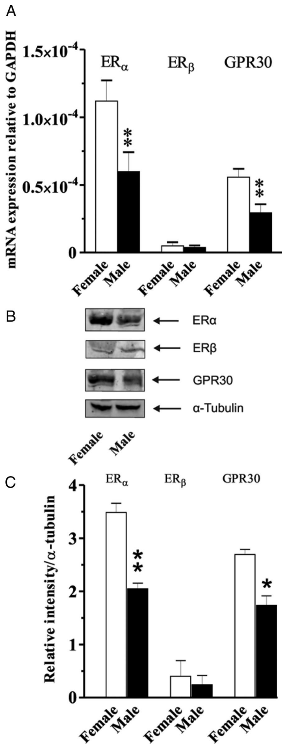
FIG. 1. A, Relative mRNA expression of ERα (n = 6 in each group), ERβ (n = 6 in each group), and GPR30 (n = 10 in each group) analyzed by qPCR in islets from female and male donors. The expression levels of ERα and GPR30 are higher in the isolated islets from female donors. B, A representative Western blot of the ERα, ERβ, and GPR30 protein expression in pancreatic islets from female and male donors. C, The mean intensity (means ± SEM) of the Western blots (n = 5 in each group) is presented as relative value of the band intensity toward the endogenous control α-tubulin. *, P < 0.05; **, P < 0.01.
