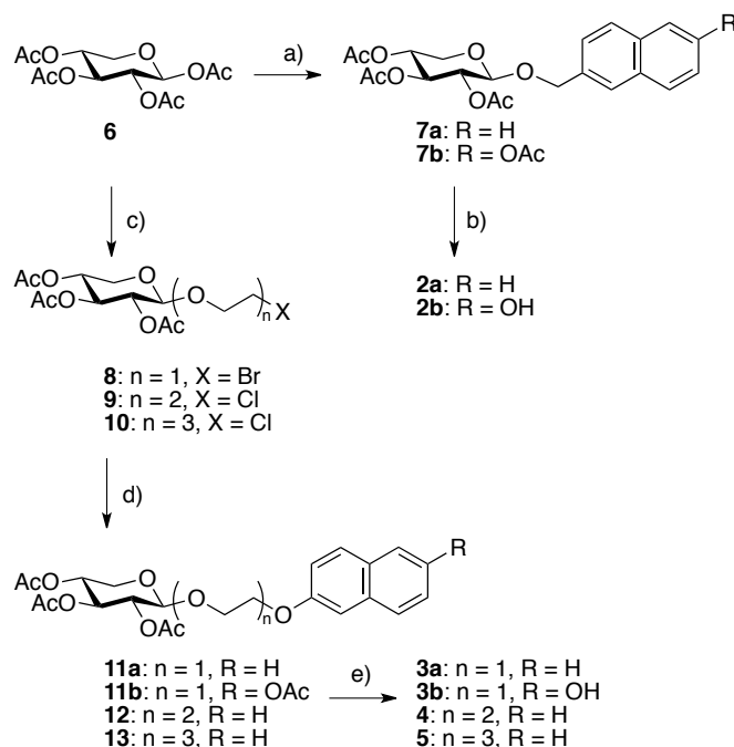
Scheme 1. Reagents and conditions: i) 6 (1.2 eq), 2-naphthalenemethanol (1 eq), BF 3 ·Et 2 O (1.5 eq), CH 2 Cl 2 , 0 °C, 7a (not isolated); 6 (1.2 eq), 6-acetoxy-2-naphthalenemethanol (1.5 eq), BF 3 ·Et 2 O (1.5 eq), CH 2 Cl 2 , 0 °C,
