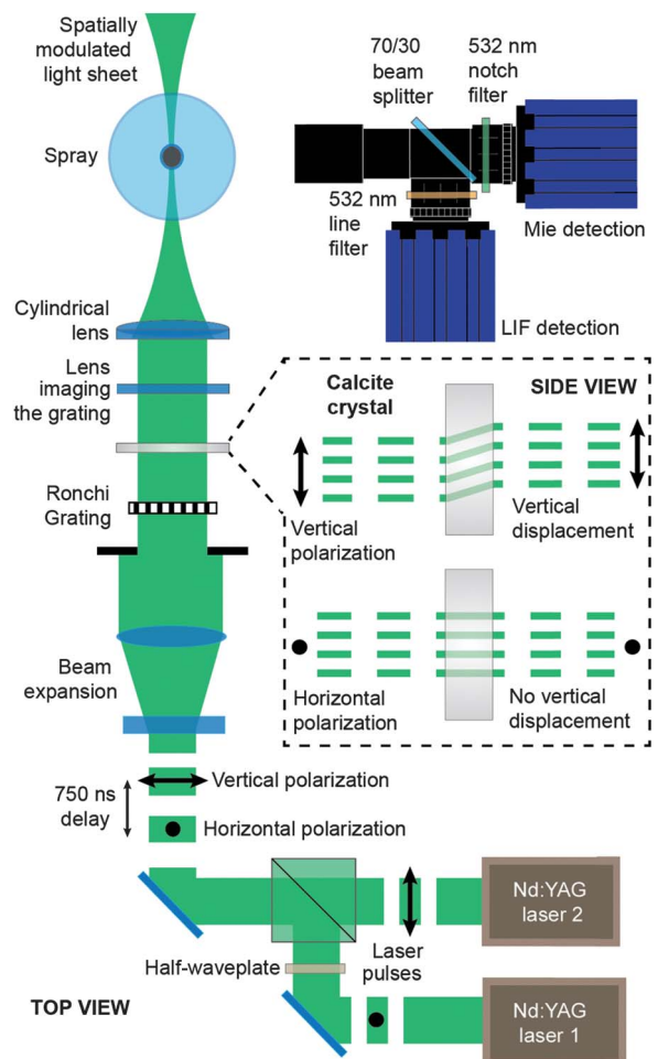
Fig. 1. Top view of the optical arrangement of 2p-SLIPI setup for simultaneous LIF and Mie detection. A spatially modulated light sheet is created by means of a Ronchi grating, while the displacement of the line pattern is operated by employing the birefringence of a calcite crystal, as illustrated in the zoomed area.
