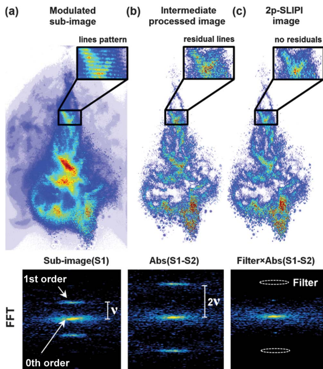
Fig. 2. Illustration of post-processing to extract a 2p-SLIPI image. (a) Sub-image for LIF detection is shown along with its FFT. (b) Intermediate image showing the absolute value of the subtraction ( I_0 - I_{180} ) and its FFT image are shown. (c) 2p-SLIPI image, along with its FFT, can be seen. A local band-rejection Gaussian filter is used for the removal of the residual lines. Note that any spray information residing within the filter range is also removed.
