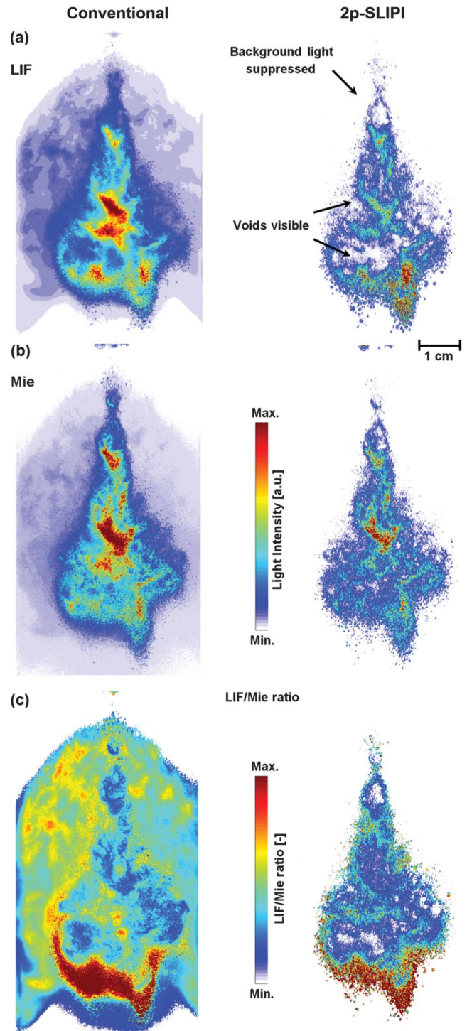
Fig. 3. Comparison between conventional light sheet imaging and 2p-SLIPI for instantaneous (a) LIF, (b) Mie scattering, and (c) LIF/Mie ratio. The transient ethanol spray is imaged at 2500 \mu\text{s} after the visible start of the injection. The 2p-SLIPI approach generates images cleaned up from multiple scattering artifacts.
