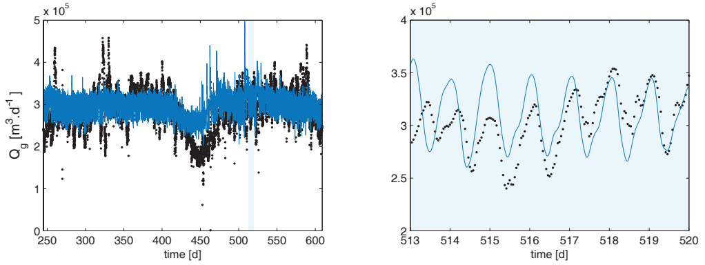
Figure 4.6: Total airflow ( Q_g ) at Käppala WWTP. Full-year simulation (left) and 7-day selection (right). Data (black markers) and model fit (blue line). The time represents simulation days, where 245 corresponds to 1 st January and 513 corresponds to 24 th October. Part of Figure 3, Paper III.
