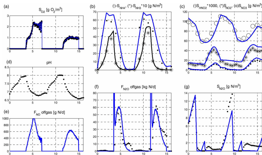
Figure 1 | Measured (markers) and simulated (solid lines) concentrations and mass flows for the nitrification/ denitrification SBR process (SBR_N/DN). Measurements of NO (e) were not available. The x-axes show time in hours.
