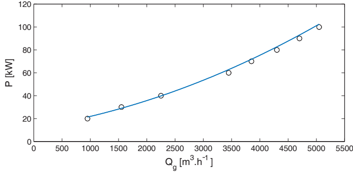
Figure 4.4: Shaft power ( P ) profile for a lobe rotor positive displacement blower (black markers) with polynomial fit (blue line) against the output airflow from the blower ( Q_g ). Figure from Arnell et al. (2013).
