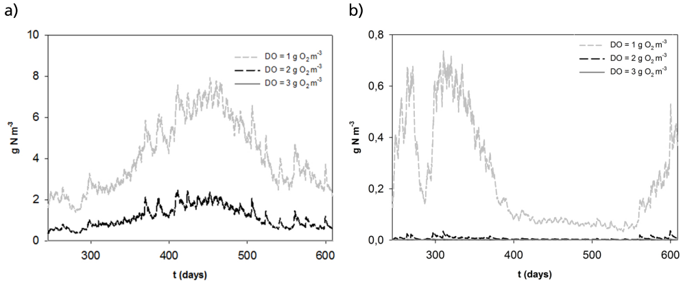
Figure 3.4: Dynamic profiles of ammonium nitrogen (left) and nitrite nitrogen (right) in the case with varying dissolved oxygen (DO) set-point. For both graphs the concentrations at \text{DO} = 3 \text{ g O}_2 \text{ m}^{-3} is zero or close to zero. Figure from Paper 1.
