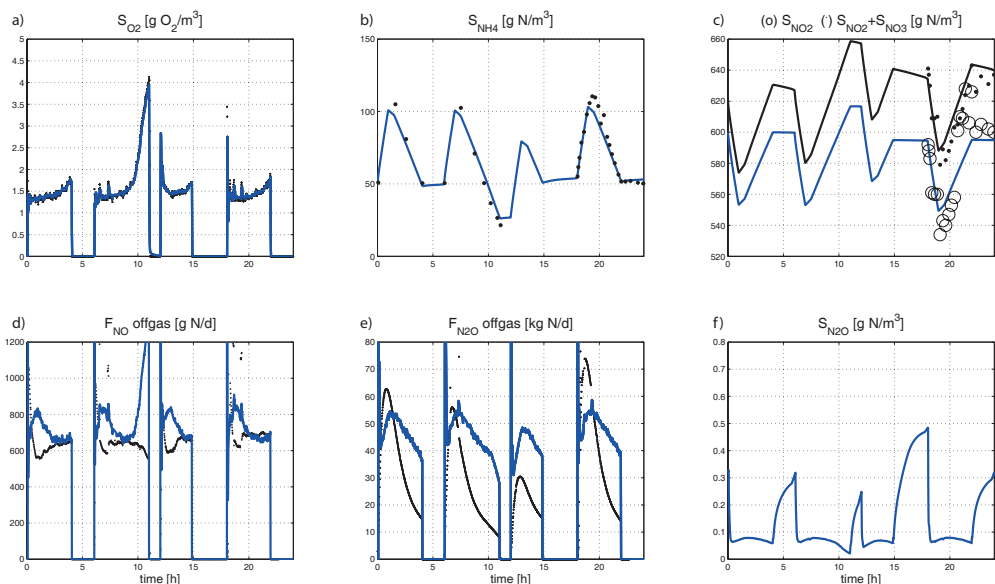
Figure 3.6: Results from the nitrification only SBR case study. a) dissolved oxygen b) ammonium c) nitrite and nitrite+nitrate d) nitrogen oxide flux to off-gas e) nitrous oxide flux to off-gas and f) dissolved nitrous oxide. Black markers represent data, blue line represents simulation results. Figure from Paper II.
