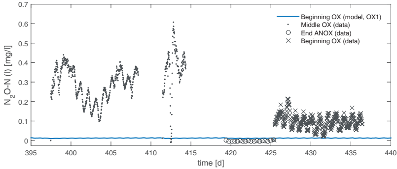
Figure 3.9: \text{N}_2\text{O} -N in aqueous phase at Käppala wastewater treatment plant. Measurements in the three different locations (grey markers) indicated in Figure 3.8 and modelled S_{\text{N}_2\text{O}} in the first aerated zone (blue line). The time scale represents simulation days, where 395 corresponds to 29 th of May. Figure from Paper vi.
