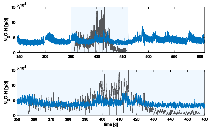
Figure 4. \text{N}_2\text{O} measurements at Käppala WWTP and model calibration result. Data – grey, model – blue. Full year simulation (top) and day 350 to 460 covering the \text{N}_2\text{O} measurement campaign (bottom).
