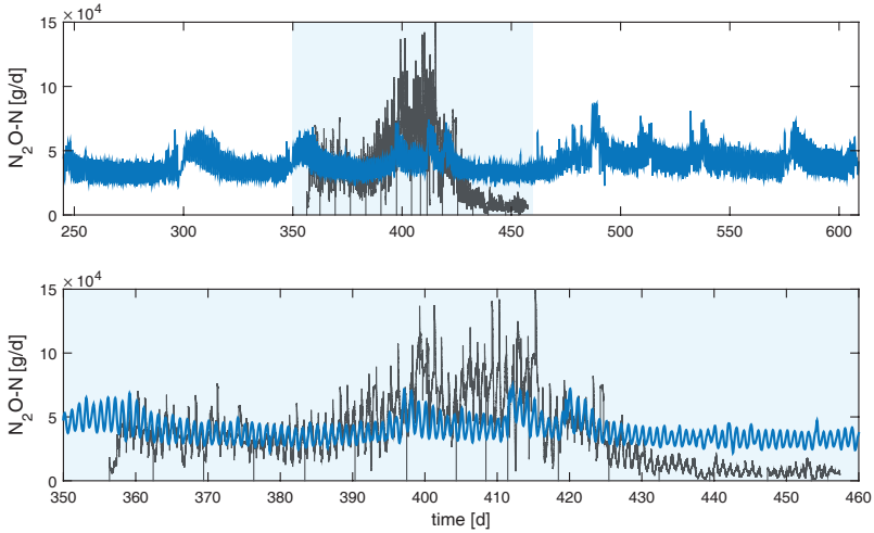
Figure 3.10: \text{N}_2\text{O} in off-gas at Käppala wastewater treatment plant. Measured data (grey line) and model result (blue line). Full year simulation (top) and day 350 to 460 covering the \text{N}_2\text{O} measurement campaign (bottom). The time represents simulation days, where 245 corresponds to 1 st January and day 350 corresponds to 14 th of April. Figure from Paper vi.
