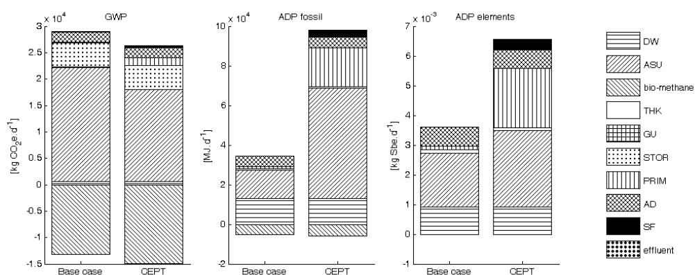
Figure 6.5: Life cycle analysis results for the base case compared to chemically enhanced primary treatment (CEPT) in three categories: Global Warming Potential (GWP), Abiotic Depletion Potential (ADP) fossil, and ADP elements. Results presented for individual unit processes: sludge dewatering unit (DW), activated sludge unit (ASU), utilisation of biomethane as vehicle fuel (biomethane), thickener (THK), biogas upgrading unit (GU), storage tank (STOR), primary clarifier (PRIM), anaerobic digester (AD), sand filter (SF) and effluent water (effluent). Figure from Paper vi.
