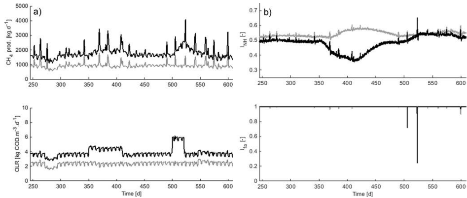
Fig. 4. Effect of AcoD on BSM2 AD process. Methane production (top left), OLR (bottom left), ammonia inhibition ( I_{NH} , top right) and LCFA inhibition ( I_{LA} , bottom right). Grey lines are standard BSM2 results without AcoD and black lines are the simulated scenario with AcoD (filtered values).
