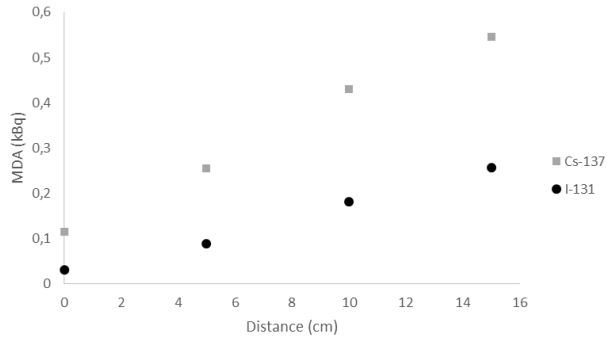
Figure 5. MDA values for the radionuclides placed at different depths in the 30 cm diameter phantom where 0 cm corresponds to the phantom surface and 15 cm to the center of the phantom.
