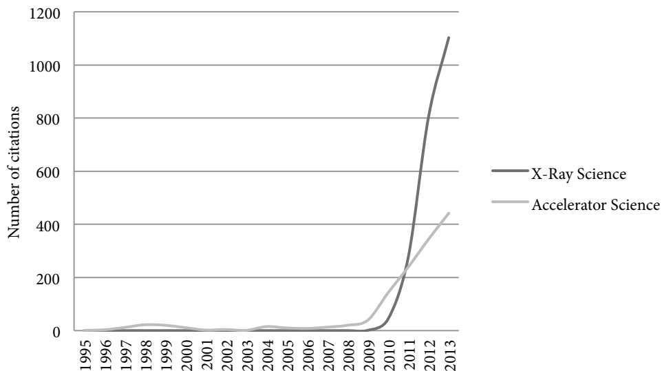
Figure 4: Citations, 1995-2013
