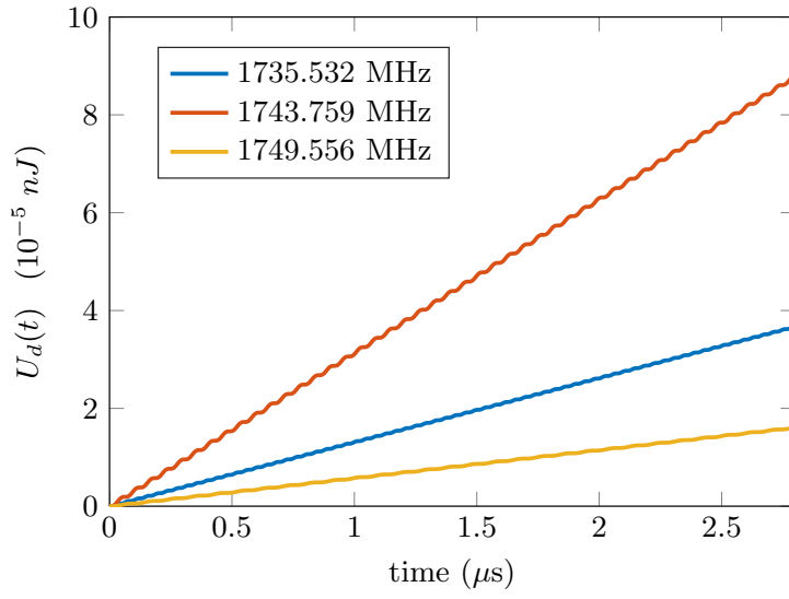
Figure 10: Evolution of the dissipated energy for the modes 18 (blue), 19 (red) and 24 (yellow) for a single bunch.
