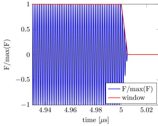
Figure 2: The input signal chosen for the simulations is a sinusoid oscillating at the \pi mode frequency (blue) modulated by a square window (red)
