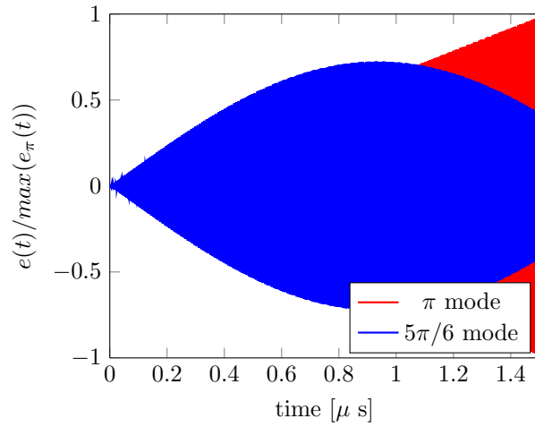
Figure 3: Evolution of the electric field amplitude of the accelerating mode (red) and of the 5\pi/6 mode (blue). The accelerating mode keeps growing while the 5\pi/6 mode reaches a maximum before decaying.
