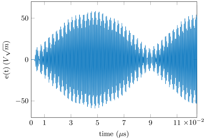
Figure 6: Evolution of the electric field excited by 40 bunches for the mode resonating at 1749.556 MHz. The curve is the first part of a simulation with 1000 bunches. The pattern repeats itself as long as there are bunches in the cavity.
