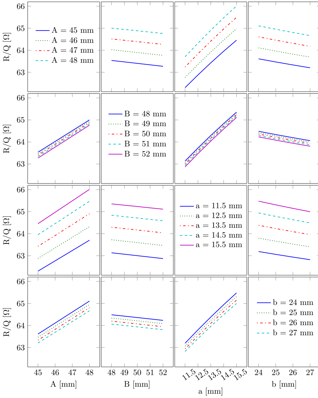
Figure 16: Interaction plot, R/Q over the geometric parameters for the inner cell design.
