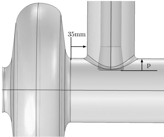
Figure 32: Coaxial coupler used in the simulations
