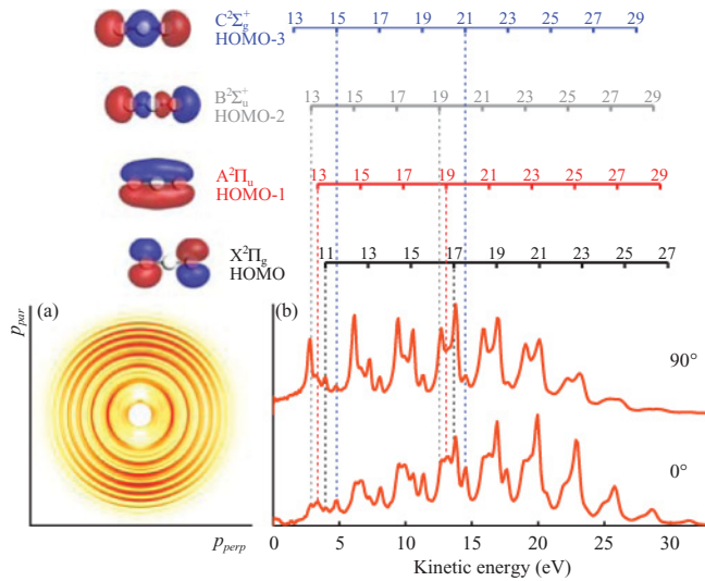
FIG. 1. (Color online) (a) Photoelectron momentum distribution for photoionization of randomly oriented CO 2 molecules by an XUV pulse generated by means of HHG and (b) photoelectron spectra for electrons emitted parallel ( \theta_{e^-} = 0^\circ ) and perpendicular ( \theta_{e^-} = 90^\circ ) to the polarization of the ionizing XUV pulse, obtained by integrating over a finite acceptance angle of \pm 20^\circ . The peaks in the spectra in panel (b) are the result of the presence of four ionization channels corresponding to the HOMO ( X^2\Pi_g^+ , I_p = 13.8 eV), the HOMO-1 ( A^2\Pi_u , I_p = 17.6 eV), the HOMO-2 ( B^2\Sigma_u^+ , I_p = 18.1 eV), and the HOMO-3 ( C^2\Sigma_g^+ , I_p = 19.4 eV) orbitals of CO 2 . Each channel can be accessed by multiple harmonic orders in the XUV pulse, which are indicated in the top part of the figure.
