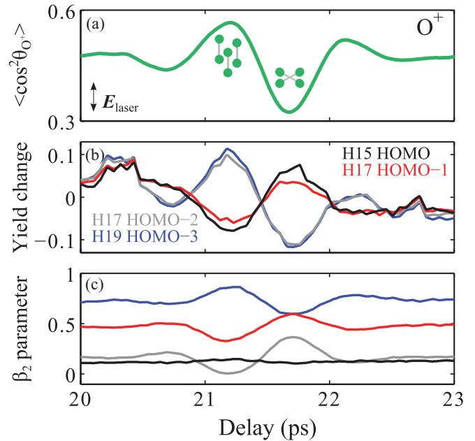
FIG. 2. (Color online) (a) \langle \cos^2 \theta_{O^+} \rangle of O + fragments as a function of the delay between the IR and XUV pulses around the second alignment revival. Channel-specific evolution of the (b) yield and (c) \beta_2 parameter of the PAD around this revival.
