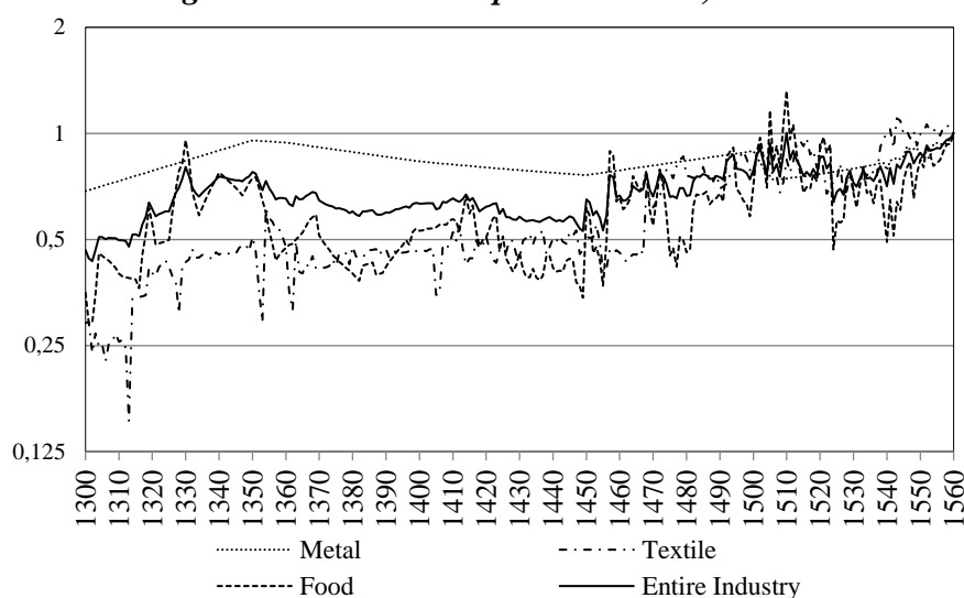
Figure 6. Industrial output 1300-1560, 1560=1
