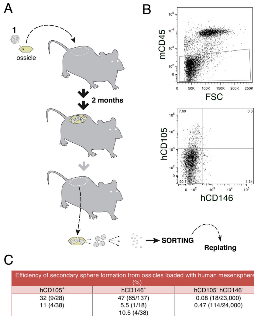
Figure S3. In Vivo Transplantation and Recovery of Human BM Mesenspheres, Related to Figure 4
