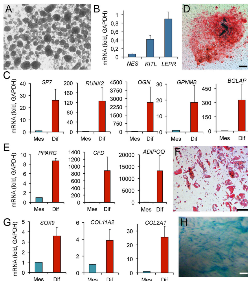
Figure 3. Human Mesenspheres Can Be Derived from Fetal BM
