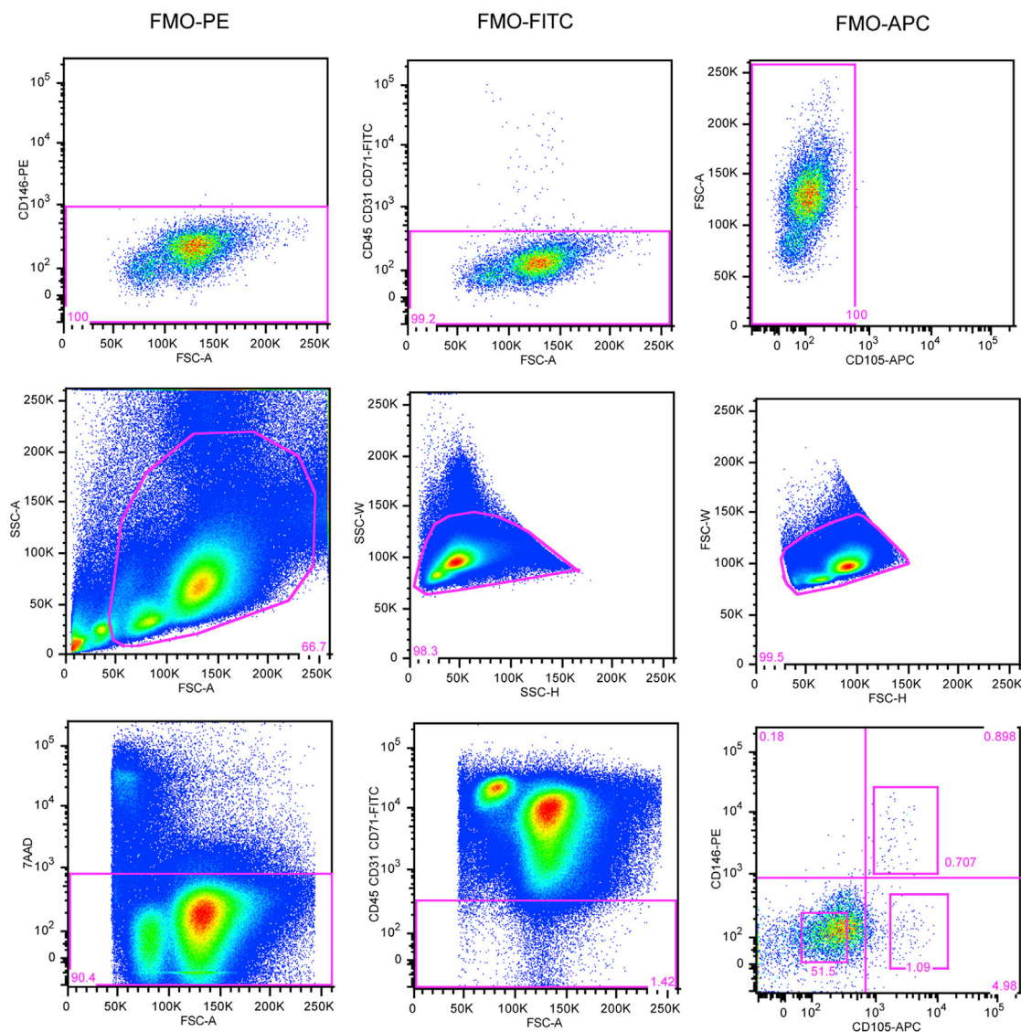
Figure S2. Human BM Mesenchymal Stem Cells (BMSCs) Are Derived from CD45 + CD31 + CD71 + CD105 + CD146 + Cells, Related to Figure 2
