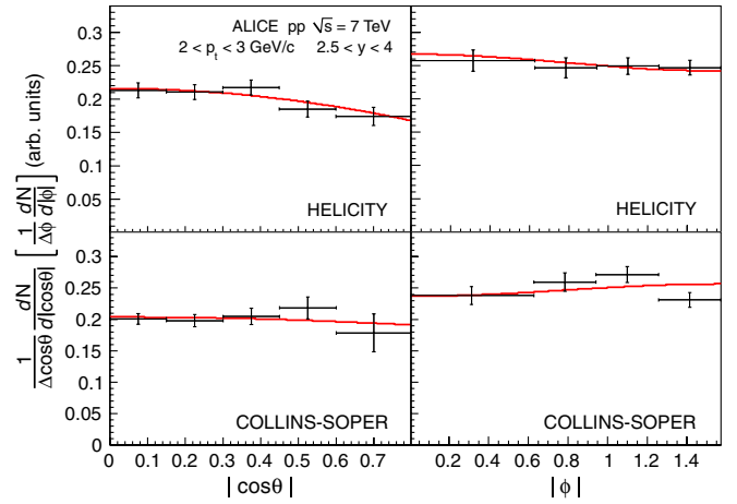
FIG. 2 (color online). The acceptance-corrected angular distributions for the J/\psi decay muons, for 2 < p_t < 3 GeV/c. The simultaneous fit to the results in the CS and HE frames is also shown. The plotted errors are purely statistical. The horizontal bars represent the bin width.
