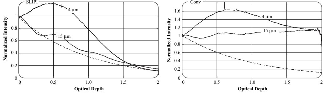
Figure 4: Cross-sections from two images where only elastically scattered light was collected, together with the decay of light intensity as predicted by the Bouguer-Beer law (dashed line). Both SLIPI and conventional data clearly show how the influence of the Mie scattering lobes make any theoretical comparisons challenging.
