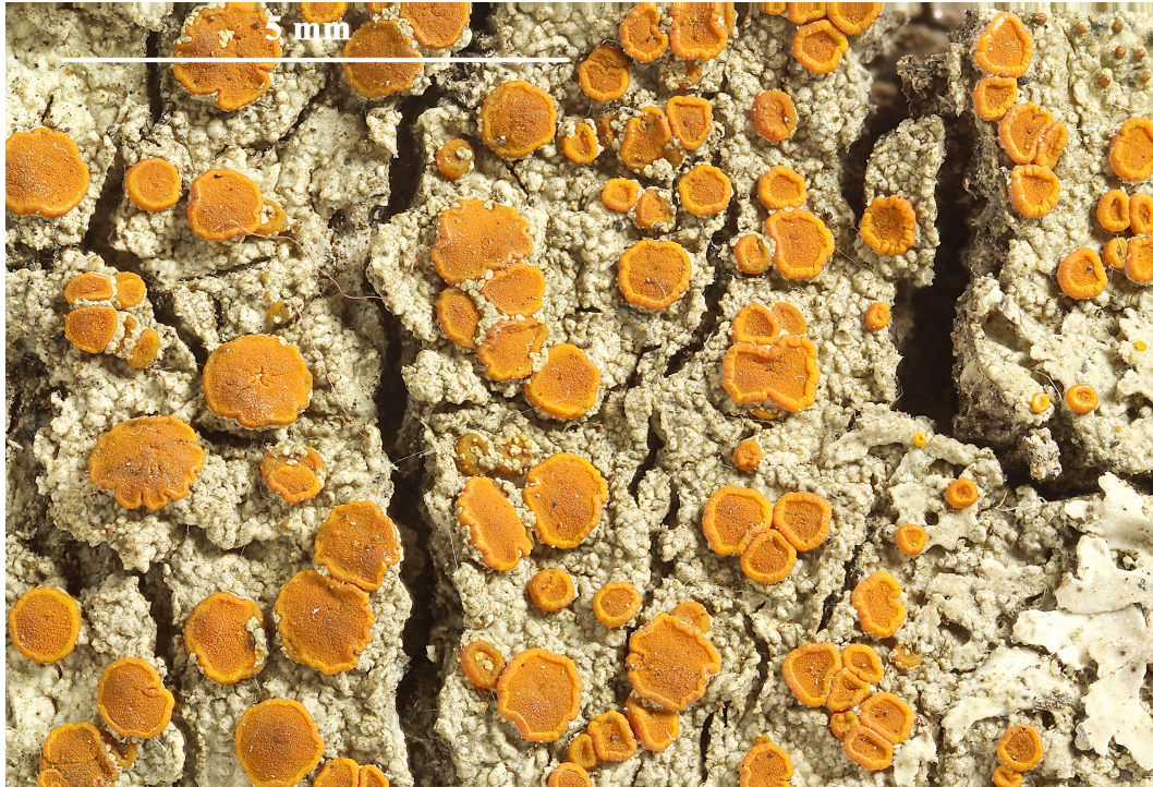
Figure 1. Eilifdahlia schwarzii (HOLOTYPE), general habit. Photo: Felix Schumm.
