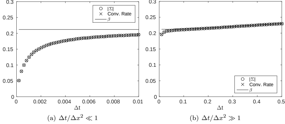
Figure 9: Semidiscrete estimator \beta , exact rate \Sigma and numerical rates over \Delta t in 1D. D_1 = 1 , D_2 = 0.5 , \lambda_1 = 0.3 and \lambda_2 = 1 , \Delta x = 1/20 . On the left: \Delta t = 1e-2/50, 2 \cdot 1e-2/50, \dots, 50 \cdot 1e-2/50 . On the right: \Delta t = 1e-2, 2 \cdot 1e-2, \dots, 50 \cdot 1e-2 .
