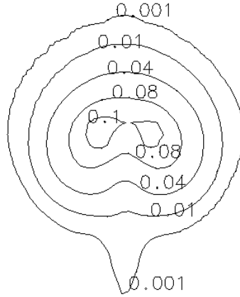
Figure 19: Diamond-shaped, (xy) plane at z/D=12
