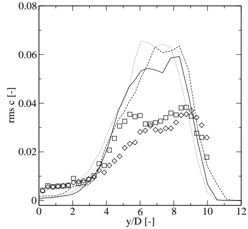
Figure 25: Computed (c) and measured (m) rms c for various nozzle shapes on a vertical line in the centerplane at z/D=8 : Round (c) —, square (m) \square , square (c) \cdots , diamond (m) \diamond , diamond (c) — —
