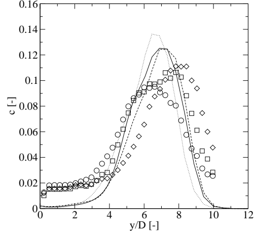
Figure 23: Computed (c) and measured (m) mean c for various nozzle shapes on a vertical line in the centerplane at z/D=8 : Round (m) \circ , round (c) —, square (m) \square , square (c) \cdots , diamond (m) \diamond , diamond (c) — —
