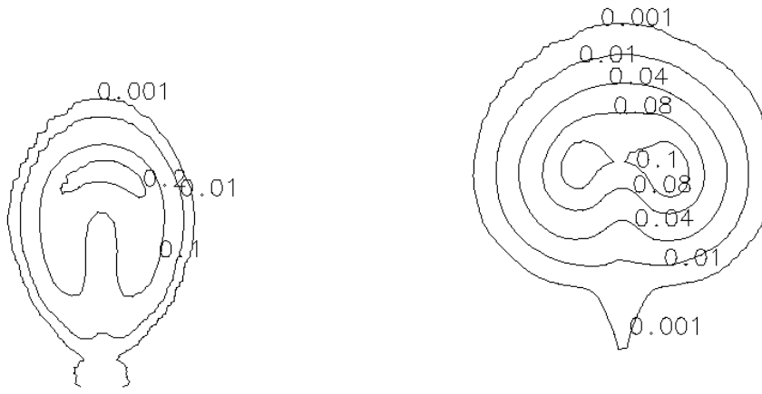
Figure 14: Circular nozzle, proximal cross-sectional (xy) plane at z/D=4
