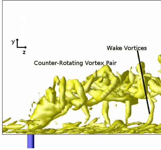
Figure 1: \lambda_2 vortex visualization [8] of the counter-rotating vortex pair and wake vortices
