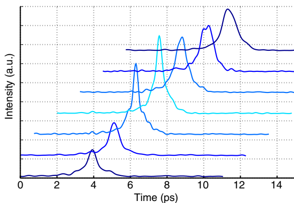
FIG. 2 (color online). A series of electro-optic signals (offset for display) collected as the electron bunch compressors at SLAC were changed, changing the bunch length. The minimum FWHM shown represents a time of 270 fs which is the resolution limit of the apparatus.
