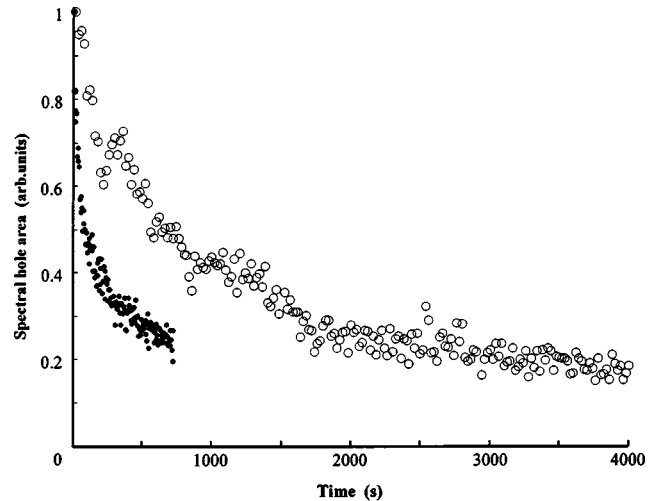
FIG. 4. Spectral hole decay in \text{Pr:Y}_2\text{SiO}_5 . The circles show the relaxation in a magnetic field of around 0.01 T. The reference curve (dots) shows the relaxation in zero magnetic field, up to 750 s after the creation of the hole. The curves do not follow single exponentials. Note, for instance, the long-lived components in both data sets.
