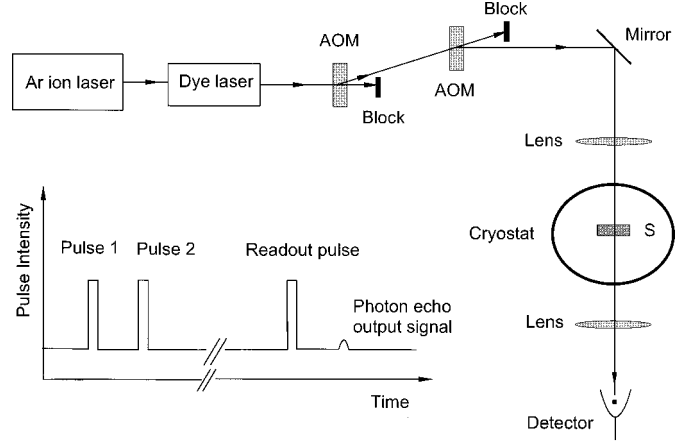
FIG. 2. Schematic view of the experimental arrangement used to compare the theoretical signal strength calculations with experimental data. The excitation pulses are switched on using two acousto-optic modulators (AOM). S is the photon-echo sample, which is placed in a cryostat to eliminate line broadening from thermal phonons. The inset schematically shows the relative timing of the excitation pulses and the echo signal.
