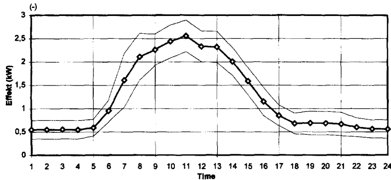
Fig. 9. Standard weekday load shape for district heated schools with kitchen, outdoor temperature above 15°C. Mean temperature – 18.3°C.
