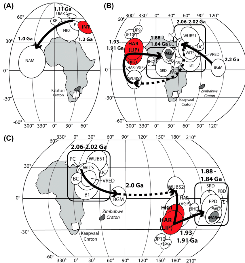
Fig. 7. A. Component INT this study (in red) compared with Mesoproterozoic poles from the Kaapvaal Craton. The 1.2–1.0 Ga segment of the Mesoproterozoic APW path is shown as a thick black arrow after Gose et al. (2013). For pole abbreviations and more details on their ages, see Table 3. B. Late Palaeoproterozoic APW path (thick black arrow) of the Kaapvaal Craton with a pre-Bushveld age for the Elim Group. C. Alternative late Palaeoproterozoic APW path (thick black arrow) for the Kaapvaal Craton with a post-Bushveld age for the Elim Group. The relative position of the Zimbabwe Craton with respect to the Kaapvaal Craton at 1.88 Ga (rotated -39^\circ around an Euler pole at 69.4^\circ\text{S} and 50.9^\circ\text{E} ; Hanson et al. 2004), is shown in both Late Palaeoproterozoic APW path options. The Zimbabwean Mashonaland sills pole (MASH) is shaded, while poles presented in this study are shown in red. APW path is stippled for times of poor data coverage.
