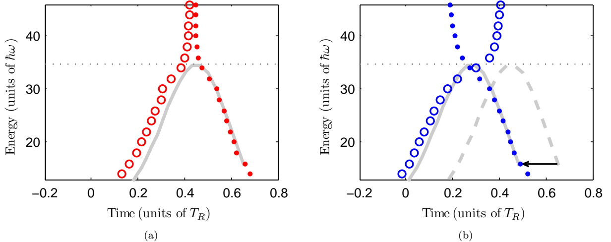
FIG. 3: (Color online) (a) The single atom response of the short ( \circ ) and the long ( \bullet ) branches are calculated using SFA for a typical IR intensity, I_R = 2 \times 10^{14} W/cm 2 . The group delays, -d\phi/d\omega , of both branches are in good agreement with the simple classical model (gray line). The group delay branches merge beyond the cut-off (dotted line). (b) The numerical in-situ scans generated using SFA with a weak blue field, I_B/I_R = 0.1\% , show qualitative agreement for both the short ( \circ ) and the long ( \bullet ) branch with the shifted simple classical model (gray line). The in-situ branches do not merge beyond the cut-off (dotted gray line).
