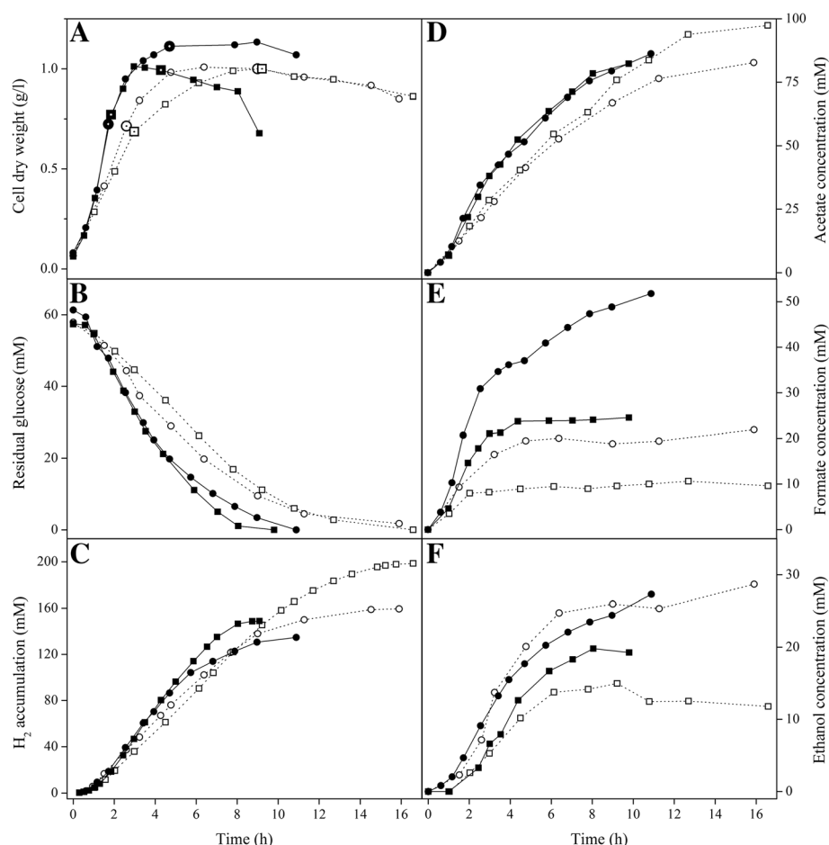
Figure 1 Growth and product formation by C. celer in pH-controlled batch fermentations performed at pH 7 and 6, with and without N_2 sparging. Growth (A), glucose consumption (B) and end product accumulation (C-F) profiles of C. celer cultured with 10 g/l glucose at pH 7 (straight lines) with N_2 sparging (Case I, filled squares) and without N_2 sparging (Case II, filled circles), and at pH 6 (dashed lines) with N_2 sparging (Case III, open squares) and without N_2 sparging (Case IV, open circles). Larger symbols in panel A represent sampling points for ATP, NADH and NAD^+ measurements. Data are from one representative fermentation per condition.
