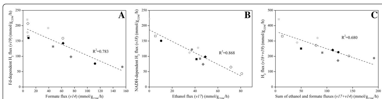
Figure 5 Correlation between formate and ethanol fluxes, and H 2 fluxes. Correlation between formate flux ( v_{14} ) and Fd-dependent H 2 flux ( v_{19} ) (A), between ethanol flux ( v_{17} ) and NADH-dependent H 2 flux ( v_{18} ) (B), and between the sum of formate and ethanol fluxes ( v_{14}+v_{17} ) and overall H 2 flux ( v_{18}+v_{19} ) (C) in exponential phase (circles), transition phase (diamonds) and stationary phase (squares) at pH 7 with N 2 sparging (Case I, black) and without N 2 sparging (Case II, dark grey), and at pH 6 with N 2 sparging (Case III, light grey) and without N 2 sparging (Case IV, white).
