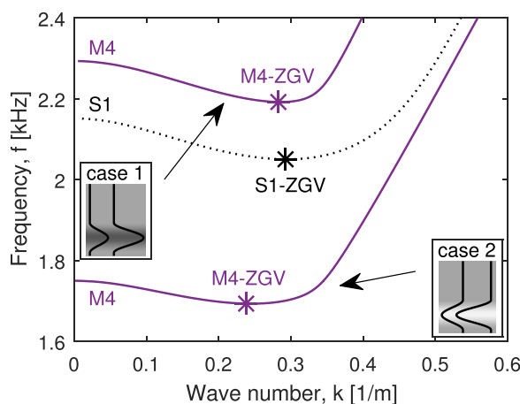
FIG. 3. (Color online) Expanded view of wave number frequency solution for the M4 mode (both case 1 and case 2) and S1 Lamb mode (isotropic reference case, dotted line). ZGV points marked with asterisks.
