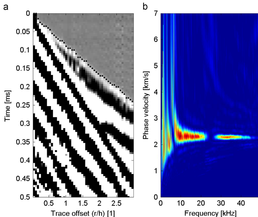
Fig. 11. Field data: (a) time domain, (b) phase velocity–frequency domain.
